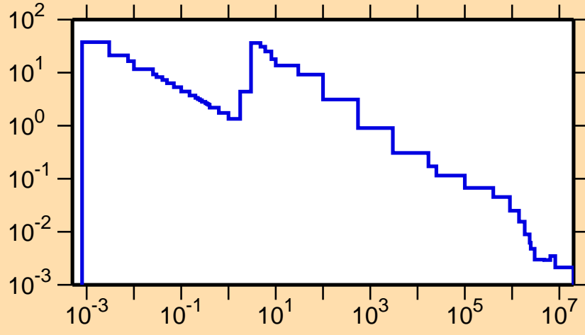
\sigma vs. E for ^{233}\text{Cm}(n,\gamma)
