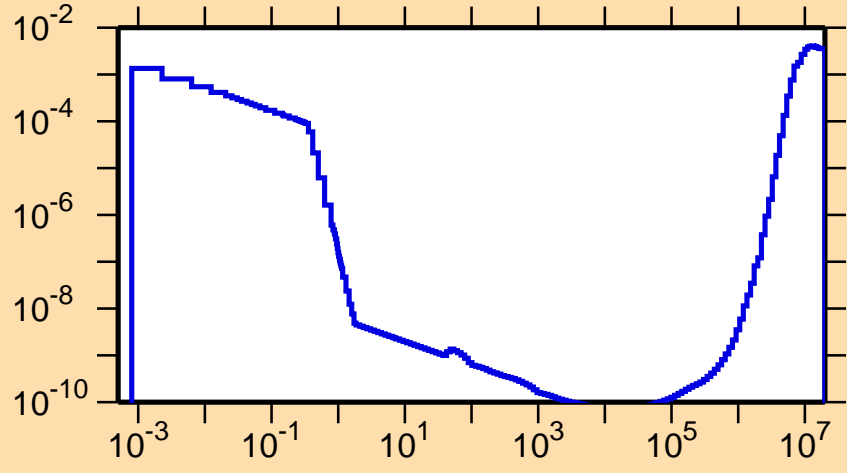
\sigma vs. E for ^{234}\text{Cm}(n,p)
