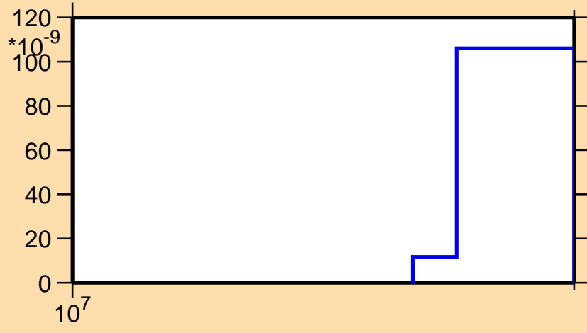
\sigma vs. E for ^{234}\text{Cm}(n,2n\alpha)
