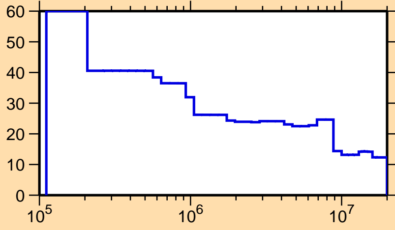
\Delta\sigma/\sigma vs. E for ^{234}\text{Cm}(n,f)
