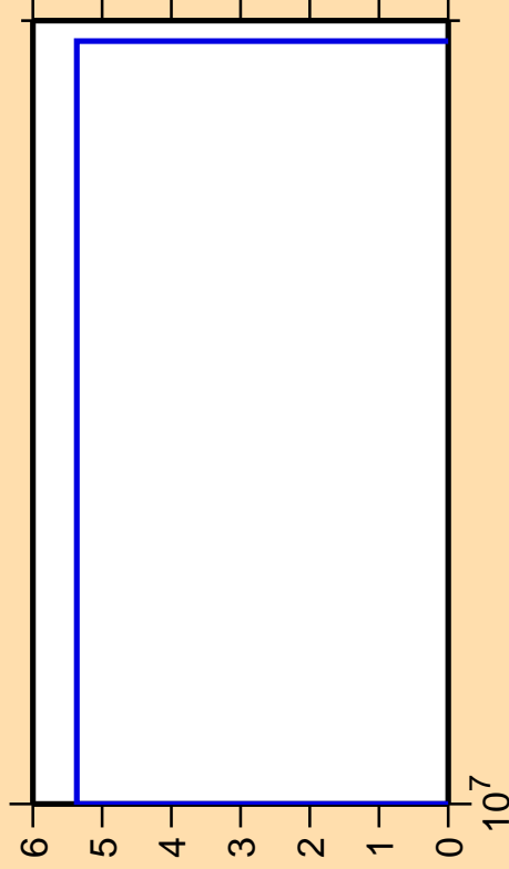
\Delta\sigma/\sigma vs. E for ^{234}\text{Cm} (mt 45)
