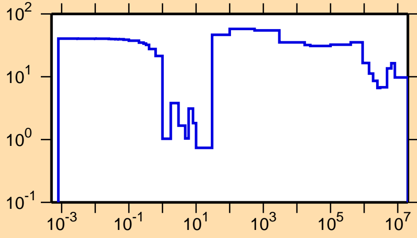
\Delta\sigma/\sigma vs. E for ^{234}\text{Cm}(n,tot.)
