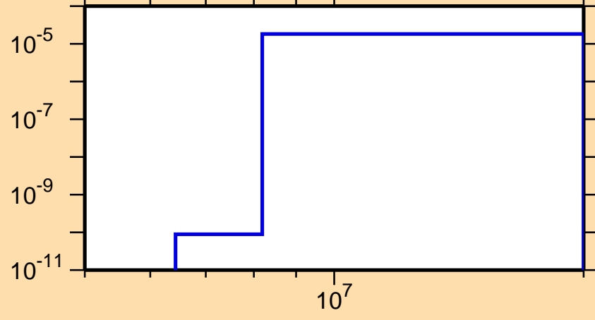
\sigma vs. E for ^{234}\text{Cm}(n,d)
