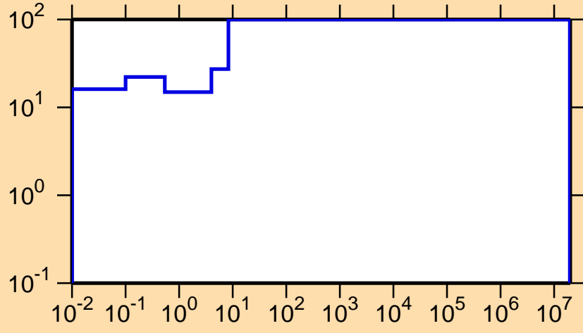
\Delta\sigma/\sigma vs. E for ^{235}\text{Cm}(n,\gamma)
