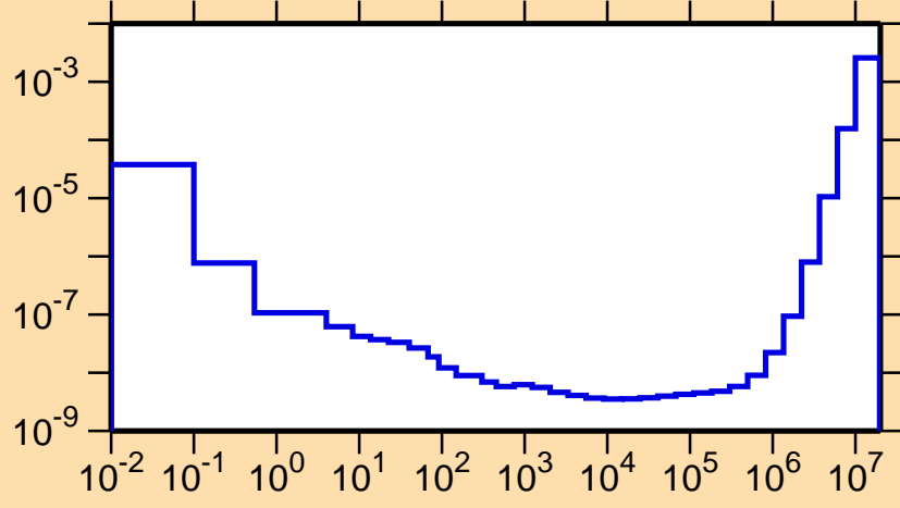
\sigma vs. E for ^{235}\text{Cm}(n,p)
