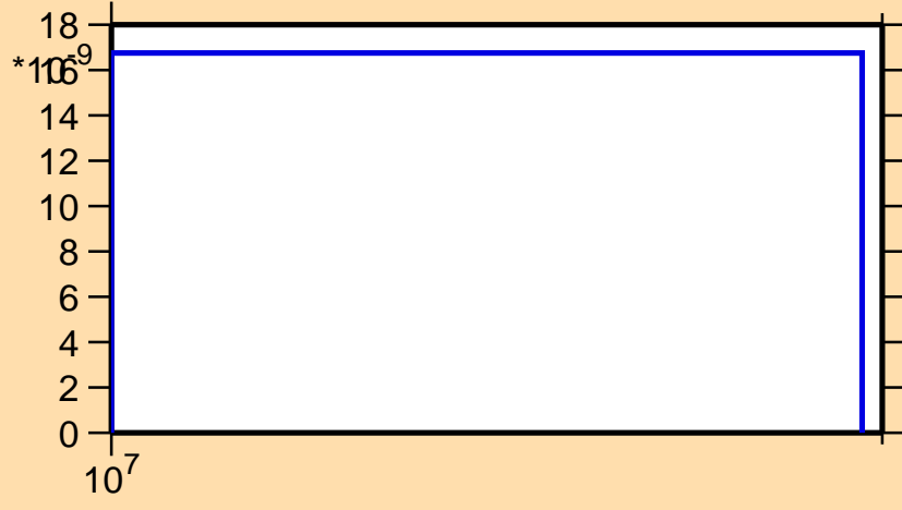
\sigma vs. E for ^{235}\text{Cm}(n,2n\alpha)
