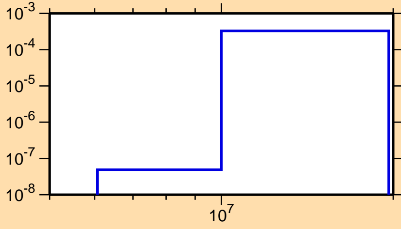
\sigma vs. E for ^{235}\text{Cm}(n,d)
