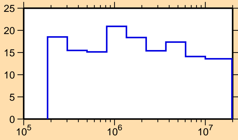
\Delta\sigma/\sigma vs. E for ^{235}\text{Cm}(n,\text{nonel.})
