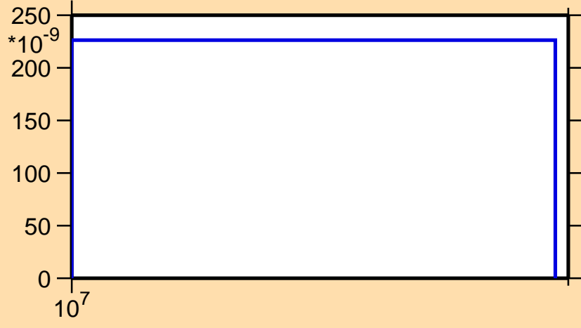
\sigma vs. E for ^{235}\text{Cm}(n,2np)
