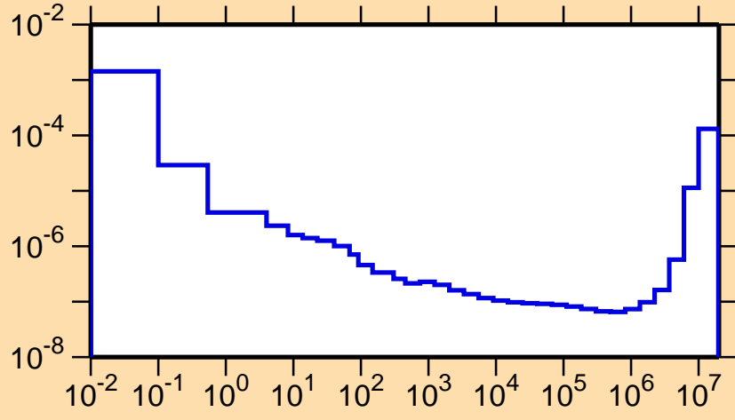
\sigma vs. E for ^{235}\text{Cm}(n,\alpha)
