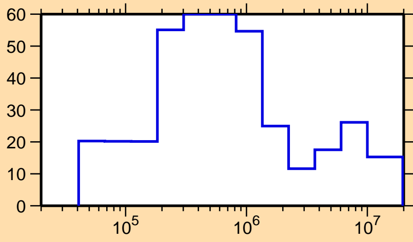
\Delta\sigma/\sigma vs. E for ^{235}\text{Cm}(n,\text{el.})
