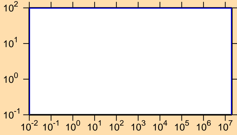
\Delta\sigma/\sigma vs. E for ^{235}\text{Cm}(n,p)
