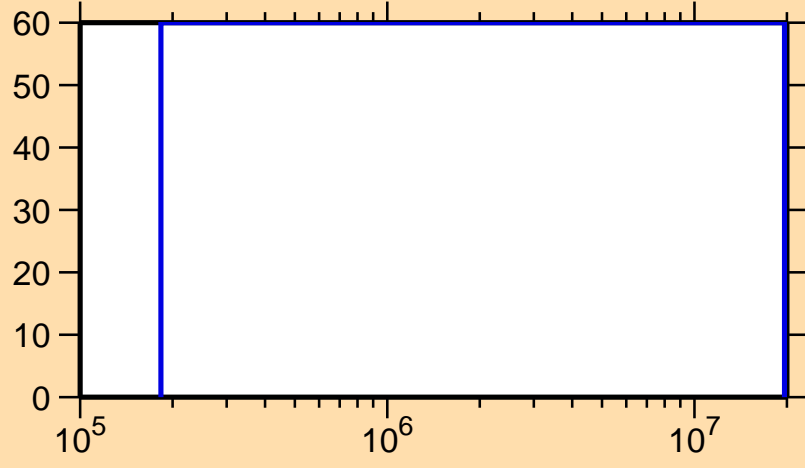
\Delta\sigma/\sigma vs. E for ^{235}\text{Cm}(n,n\text{cont.})
