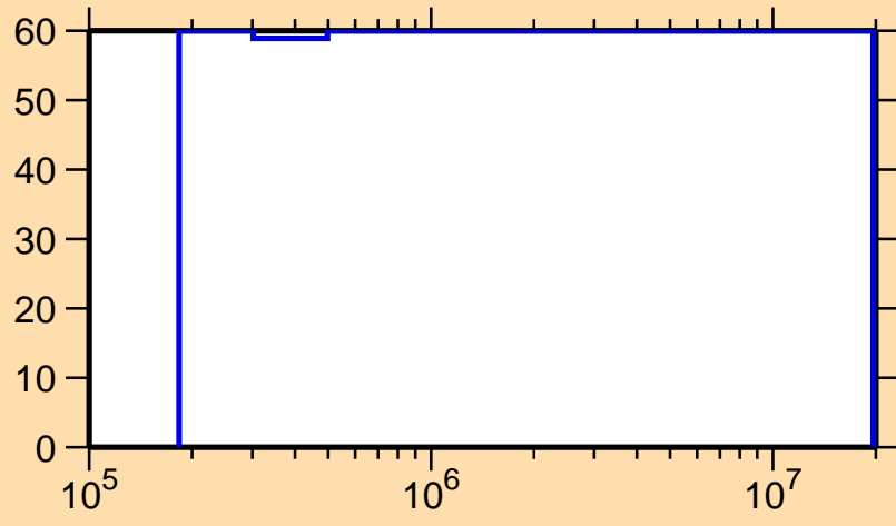
\Delta\sigma/\sigma vs. E for ^{235}\text{Cm}(n,\text{inel.})
