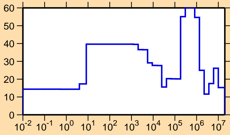
\Delta\sigma/\sigma vs. E for ^{235}\text{Cm}(n,el.)
