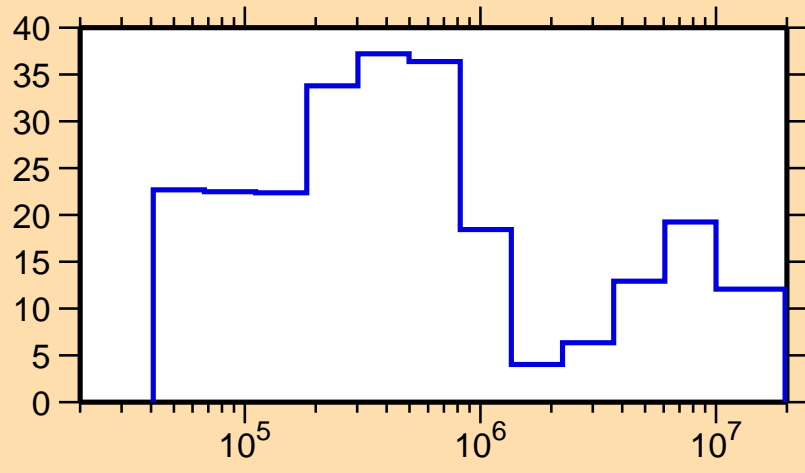
\Delta\sigma/\sigma vs. E for ^{235}\text{Cm}(n,\text{tot.})
