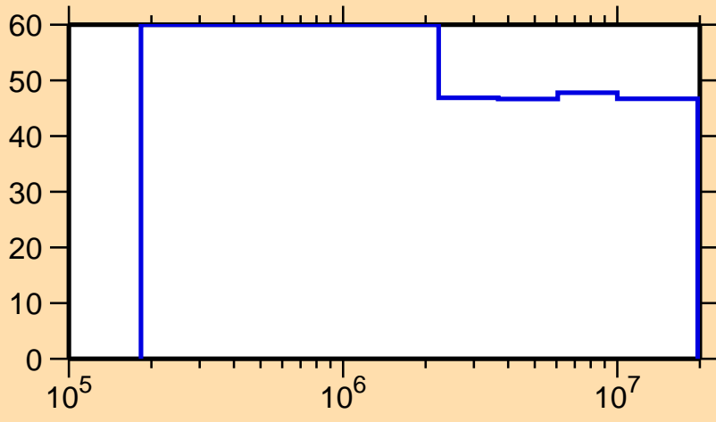
\Delta\sigma/\sigma vs. E for ^{235}\text{Cm}(n,n_1)
