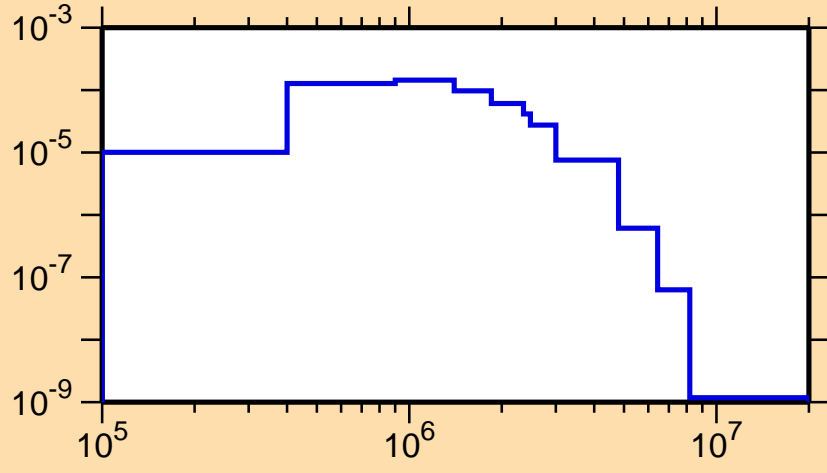
\sigma vs. E for ^{235}\text{Cm}(n,n_2)
