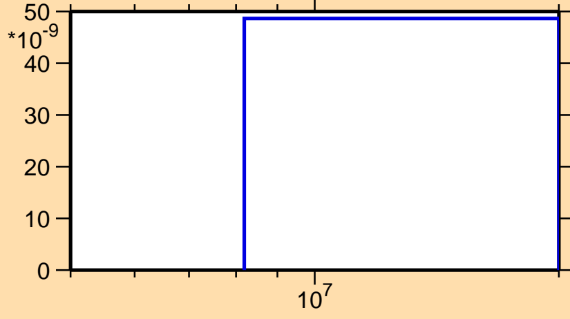
\sigma vs. E for ^{235}\text{Cm}(n,nd)
