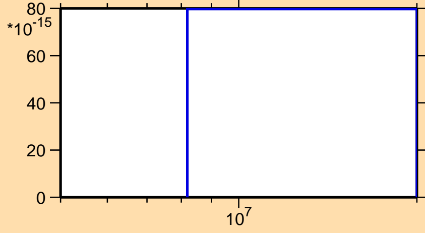
\sigma vs. E for ^{235}\text{Cm} (mt 34)
