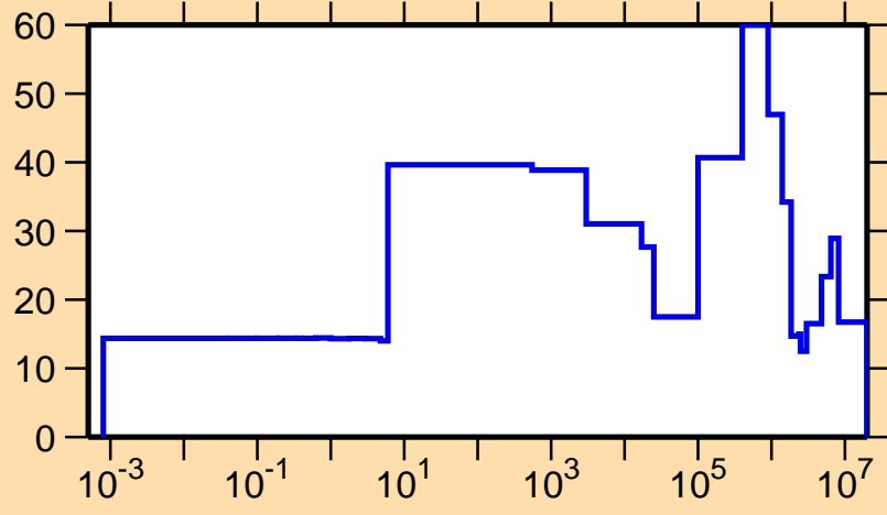
\Delta\sigma/\sigma vs. E for ^{235}\text{Cm}(n,el.)
