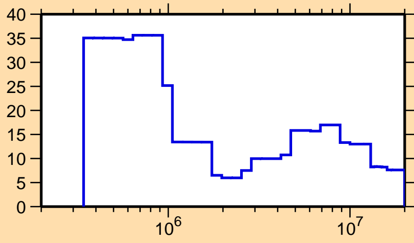
\Delta\sigma/\sigma vs. E for ^{236}\text{Cm}(n,\text{tot.})
