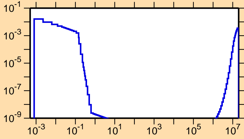
\sigma vs. E for ^{236}\text{Cm}(n,\alpha)
