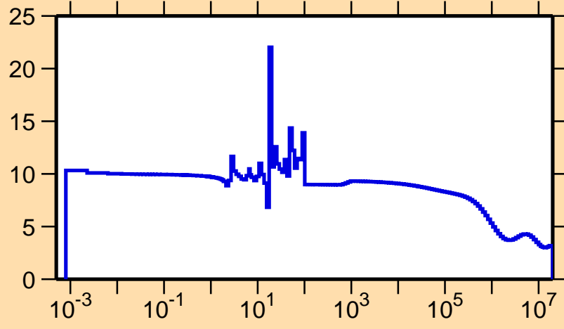
\sigma vs. E for ^{236}\text{Cm}(n,\text{el.})
