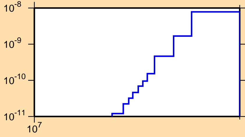
\sigma vs. E for ^{236}\text{Cm}(n,p\alpha)
