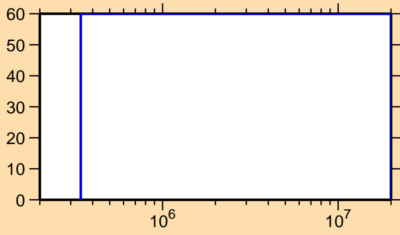
\Delta\sigma/\sigma vs. E for ^{236}\text{Cm}(n,n_1)
