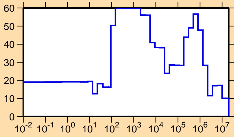
\Delta\sigma/\sigma vs. E for ^{236}\text{Cm}(n,el.)
