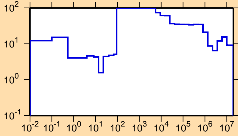
\Delta\sigma/\sigma vs. E for ^{236}\text{Cm}(n,tot.)
