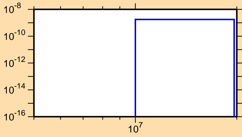
\sigma vs. E for ^{236}\text{Cm}(n,\text{He3})
