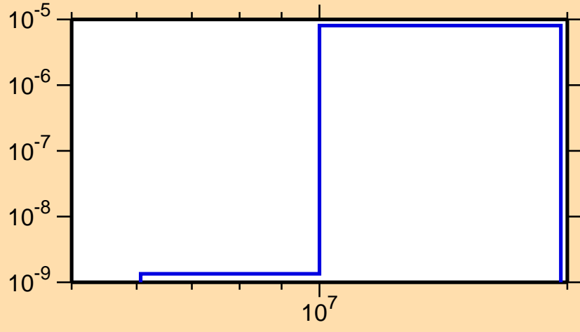
\sigma vs. E for ^{236}\text{Cm}(n,d)
