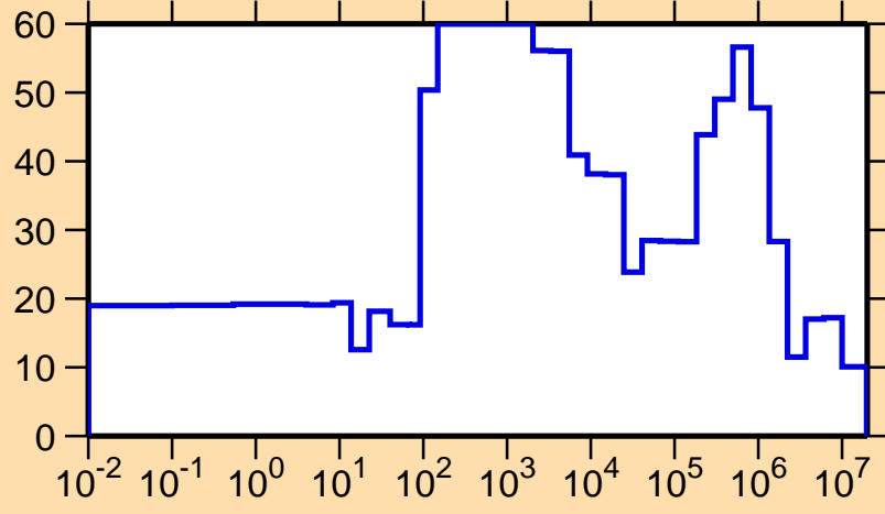
\Delta\sigma/\sigma vs. E for ^{236}\text{Cm}(n,el.)
