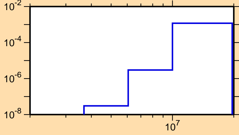
\sigma vs. E for ^{236}\text{Cm}(n,n\alpha)
