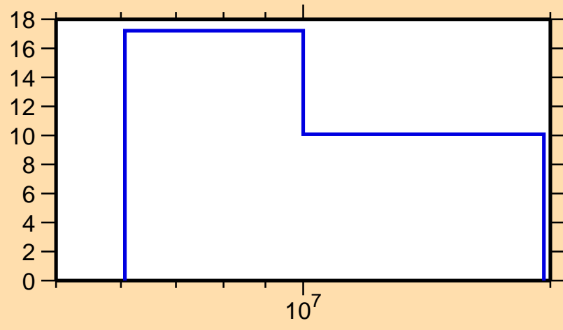
\Delta\sigma/\sigma vs. E for ^{236}\text{Cm}(n,\text{el.})
