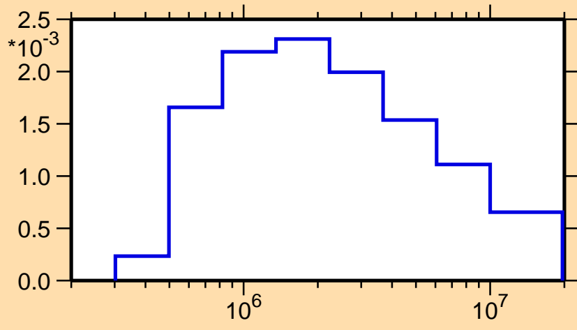
\sigma vs. E for ^{236}\text{Cm}(n,n_2)
