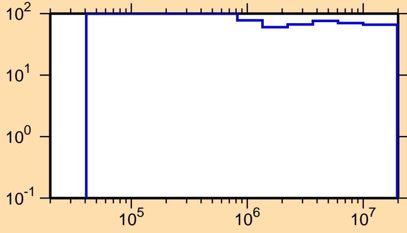
\Delta\sigma/\sigma vs. E for ^{236}\text{Cm}(n,n_1)
