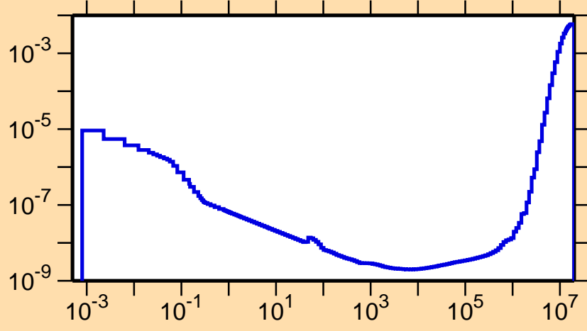
\sigma vs. E for ^{237}\text{Cm}(n,p)
