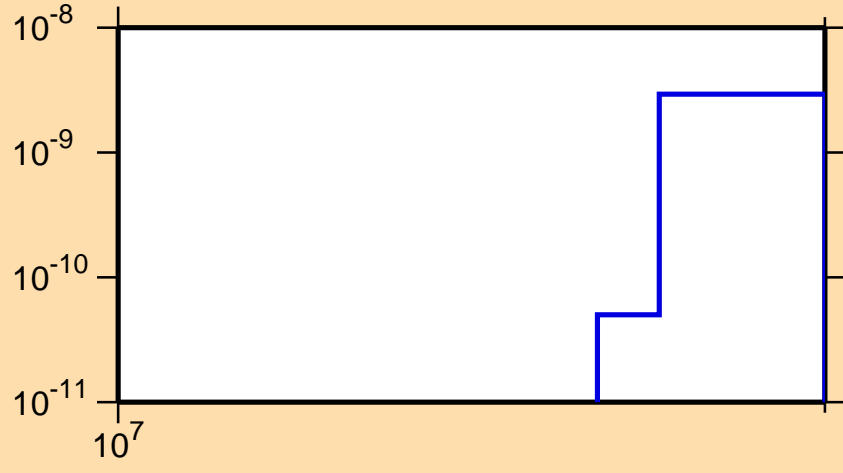
\sigma vs. E for ^{238}\text{Cm}(n,nt)
