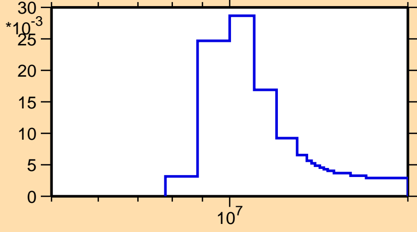
\sigma vs. E for ^{238}\text{Cm}(n,2n)
