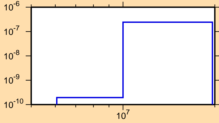
\sigma vs. E for ^{238}\text{Cm}(n,np)
