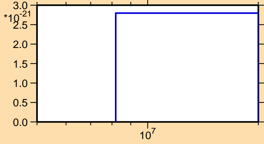
\sigma vs. E for ^{238}\text{Cm} (mt 42)
