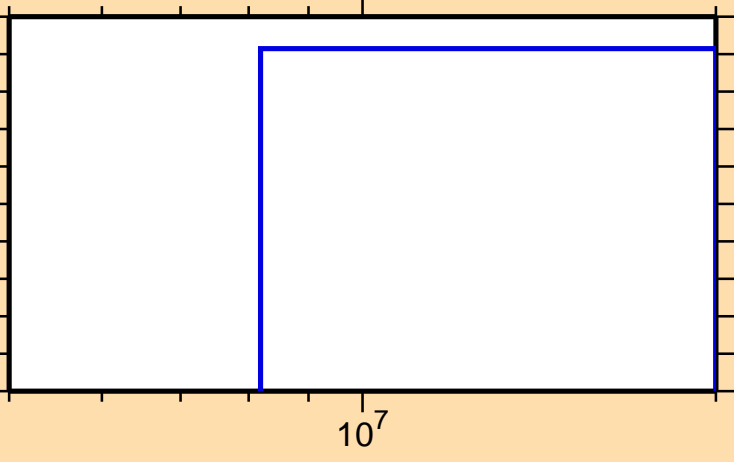
\sigma vs. E for ^{238}\text{Cm}(n,2np)
