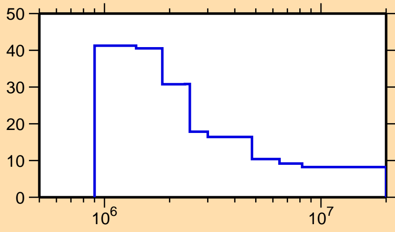
\Delta\sigma/\sigma vs. E for ^{238}\text{Cm}(n,f)
