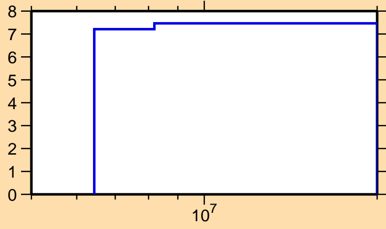
\Delta\sigma/\sigma vs. E for ^{238}\text{Cm}(n,\text{nonel.})
