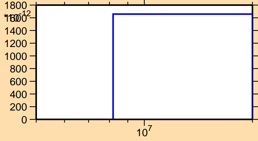
\sigma vs. E for ^{238}\text{Cm}(n,nd)
