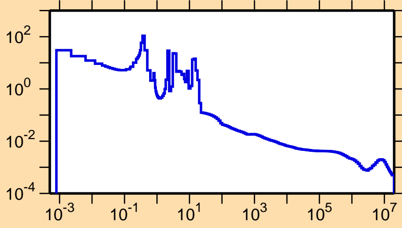
\sigma vs. E for ^{239}\text{Cm}(n,\gamma)
