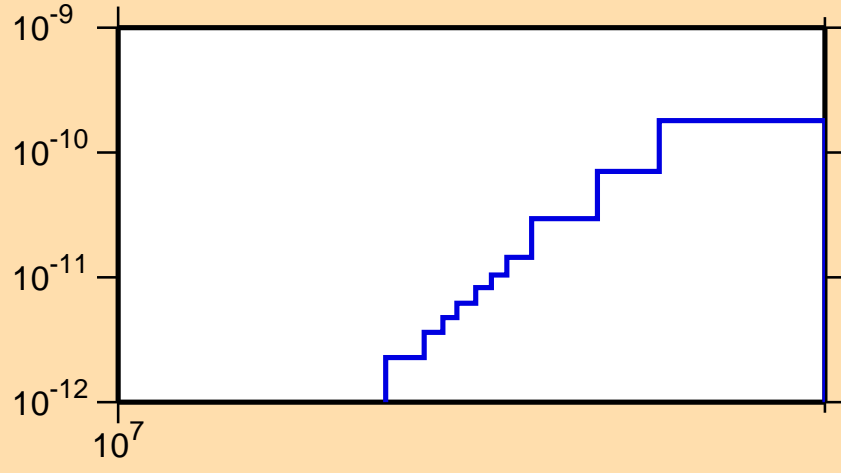
\sigma vs. E for ^{239}\text{Cm}(n,p\alpha)
