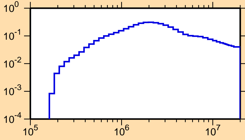
\sigma vs. E for ^{239}\text{Cm}(n,\text{inel.})
