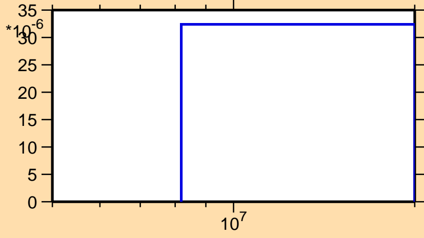
\sigma vs. E for ^{239}\text{Cm}(n,t)
