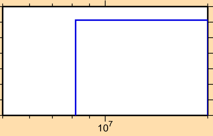
\sigma vs. E for ^{239}\text{Cm}(n,nt)
