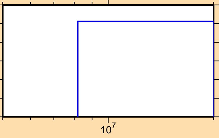
\sigma vs. E for ^{239}\text{Cm}(\text{mt117})
