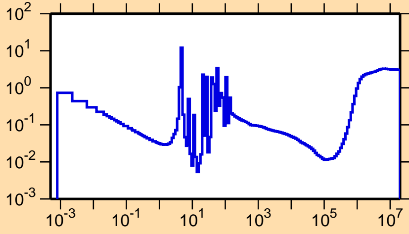
\sigma vs. E for ^{240}\text{Cm}(n,f)
