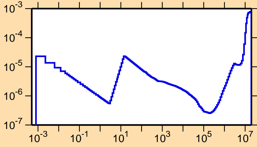
\sigma vs. E for ^{240}\text{Cm}(n,\alpha)
