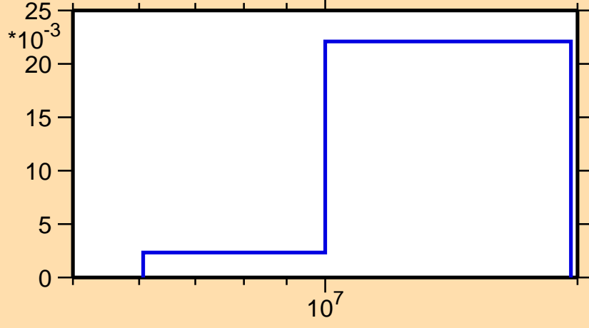
\sigma vs. E for ^{240}\text{Cm}(n,2n)
