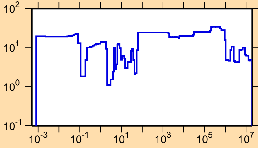
\Delta\sigma/\sigma vs. E for ^{241}\text{Cm}(n,tot.)
