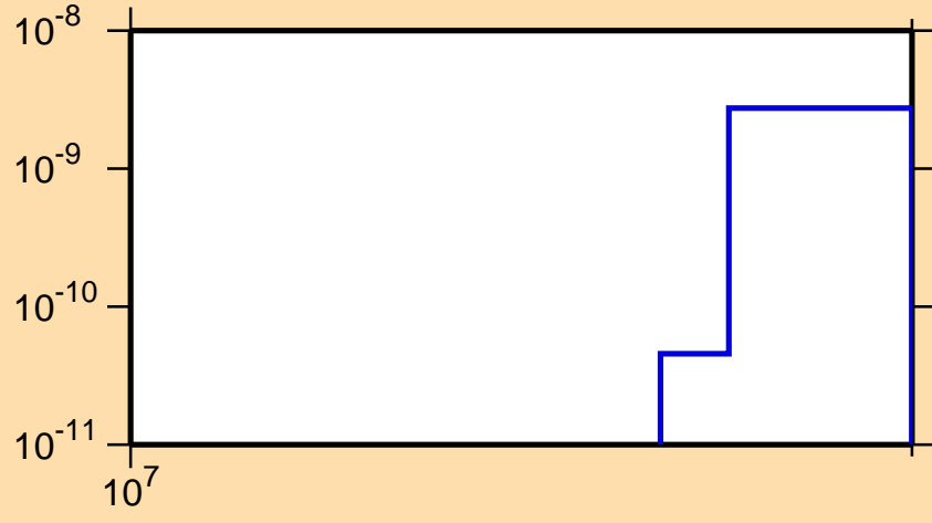
\sigma vs. E for ^{241}\text{Cm}(n,nt)
