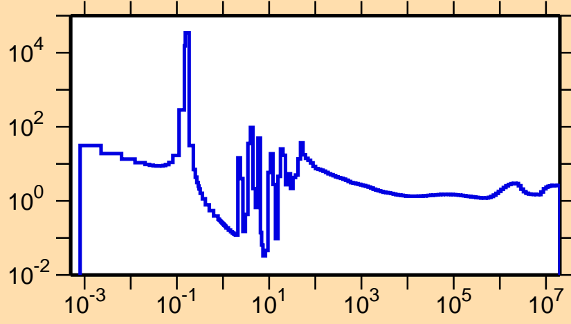
\sigma vs. E for ^{241}\text{Cm}(n,f)
