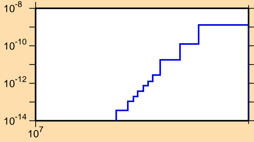
\sigma vs. E for ^{241}\text{Cm}(n,\text{He3})
