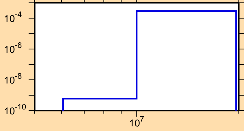
\sigma vs. E for ^{241}\text{Cm}(n,d)
