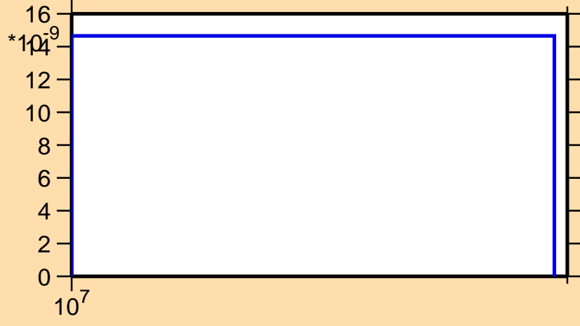
\sigma vs. E for ^{241}\text{Cm}(n,nd)
