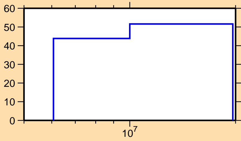
\Delta\sigma/\sigma vs. E for ^{241}\text{Cm}(n,2n)
