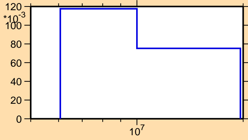
\sigma vs. E for ^{241}\text{Cm}(n,2n)
