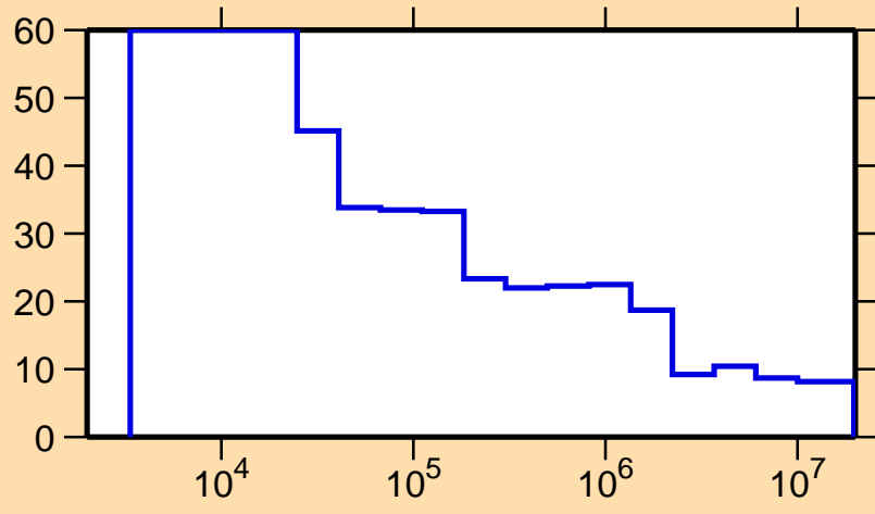
\Delta\sigma/\sigma vs. E for ^{241}\text{Cm}(n,\text{nonel.})
