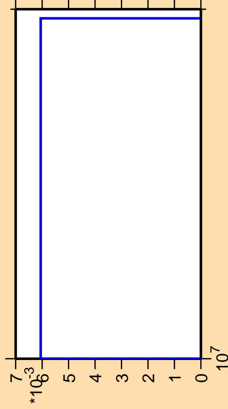
\Delta\sigma/\sigma vs. E for ^{241}\text{Cm} (mt 34)
