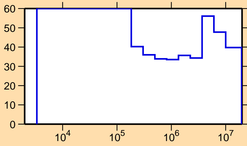
\Delta\sigma/\sigma vs. E for ^{241}\text{Cm}(n,n_1)
