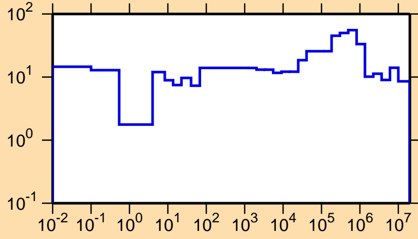
\Delta\sigma/\sigma vs. E for ^{241}\text{Cm}(n,el.)
