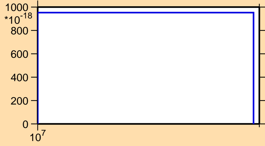
\sigma vs. E for ^{241}\text{Cm} (mt 34)
