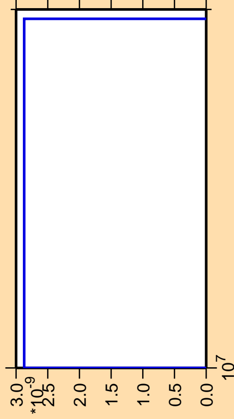
\Delta\sigma/\sigma vs. E for ^{241}\text{Cm} (mt 42)
