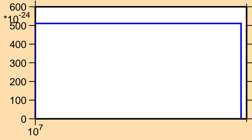
\sigma vs. E for ^{241}\text{Cm} (mt 42)
