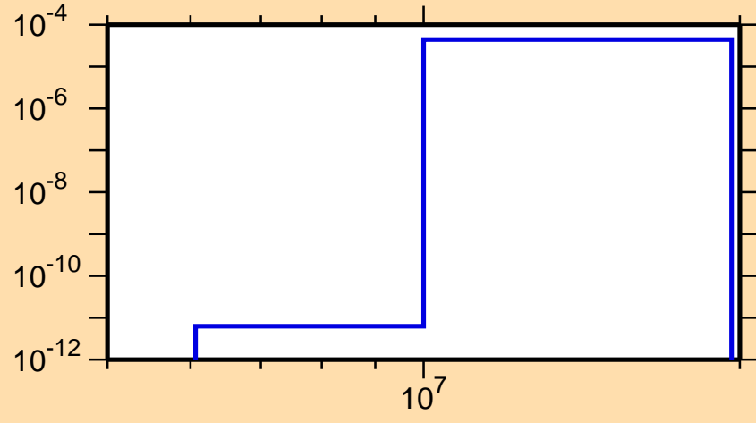
\sigma vs. E for ^{241}\text{Cm}(n,t)
