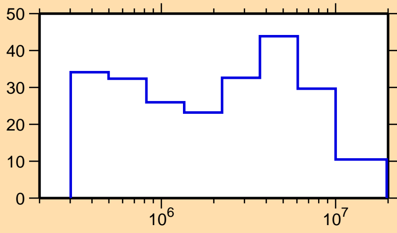
\Delta\sigma/\sigma vs. E for ^{241}\text{Cm}(n,f)
