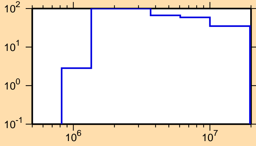
\Delta\sigma/\sigma vs. E for ^{241}\text{Cm}(n,p)
