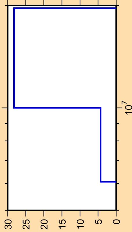
\Delta\sigma/\sigma vs. E for ^{241}\text{Cm}(n,t)
