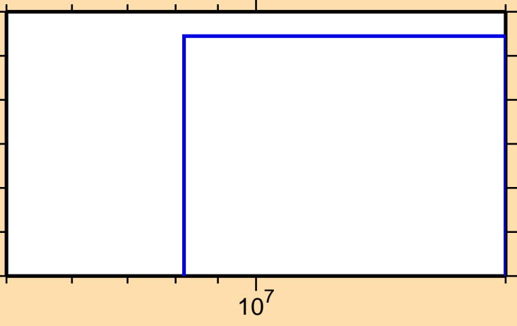
\sigma vs. E for ^{241}\text{Cm}(n,2n\alpha)
