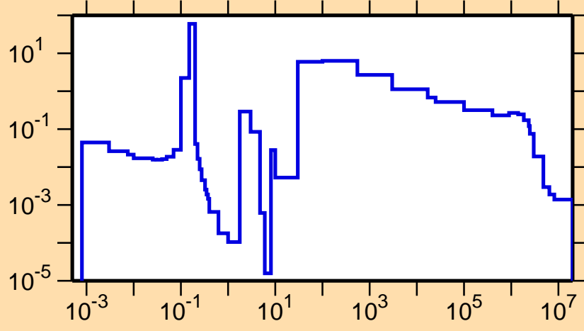
\sigma vs. E for ^{241}\text{Cm}(n,\gamma)
