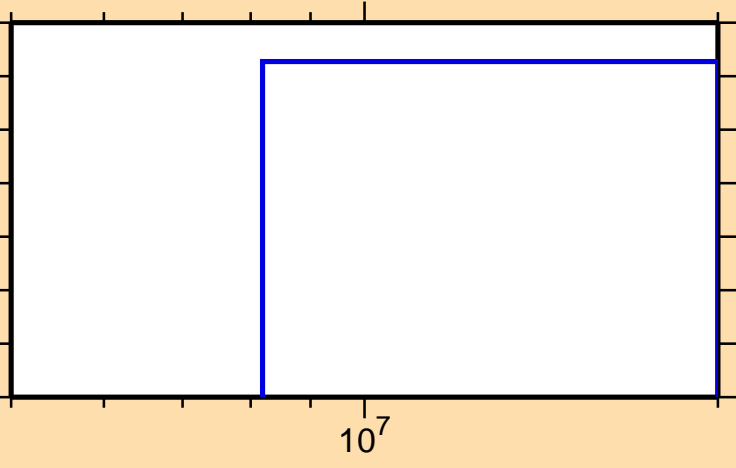
\sigma vs. E for ^{241}\text{Cm}(n,nd)
