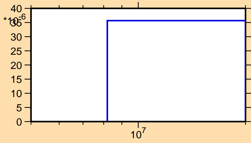
\sigma vs. E for ^{241}\text{Cm}(n,t)
