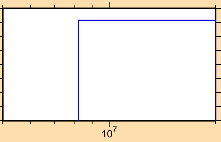
\sigma vs. E for ^{241}\text{Cm}(n,t)
