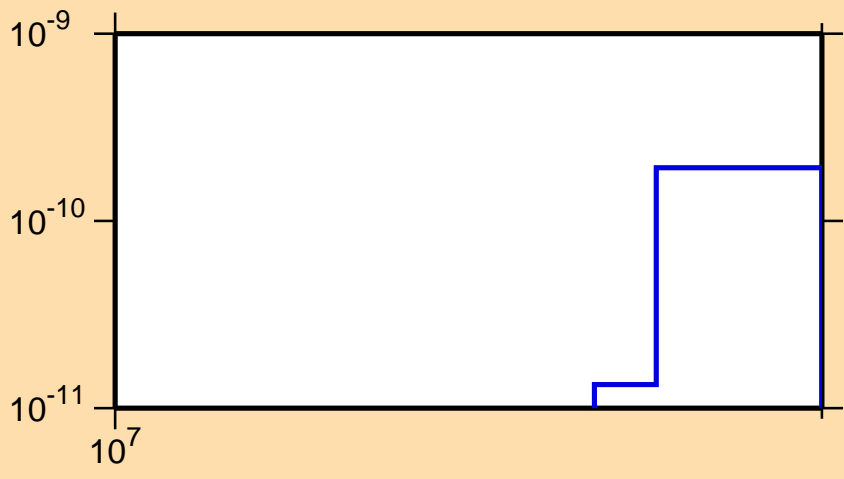
\sigma vs. E for ^{242}\text{Cm}(n,\text{He3})
