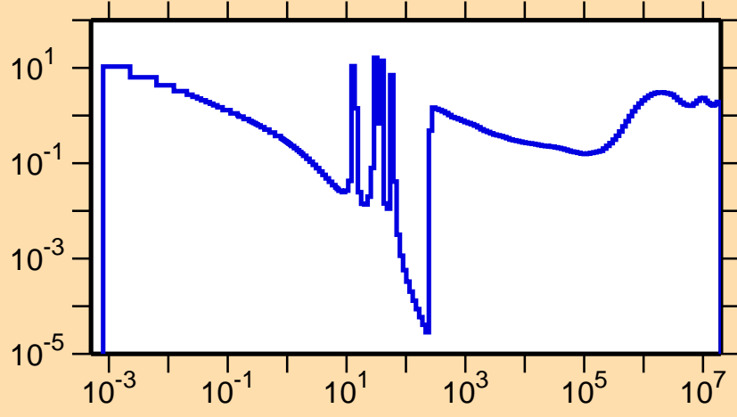
\sigma vs. E for ^{242}\text{Cm}(n,f)
