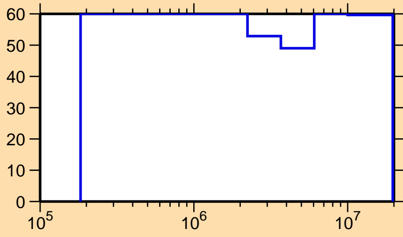
\Delta\sigma/\sigma vs. E for ^{242}\text{Cm}(n,ncont.)
