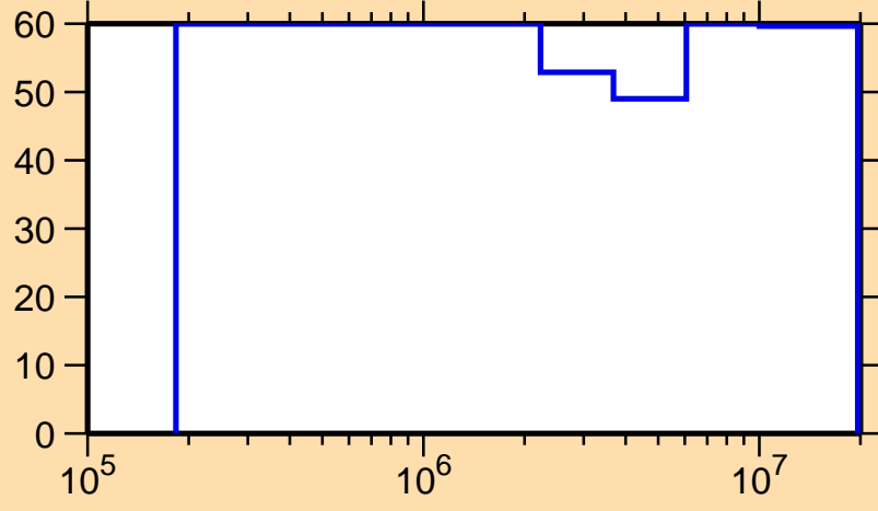
\Delta\sigma/\sigma vs. E for ^{242}\text{Cm}(n,n\text{cont.})
