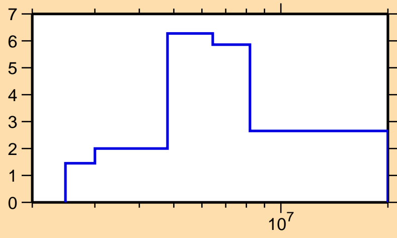
\Delta\sigma/\sigma vs. E for ^{242}\text{Cm}(n,\text{tot.})
