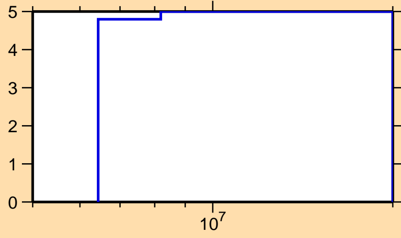
\Delta\sigma/\sigma vs. E for ^{242}\text{Cm}(n,\text{nonel.})
