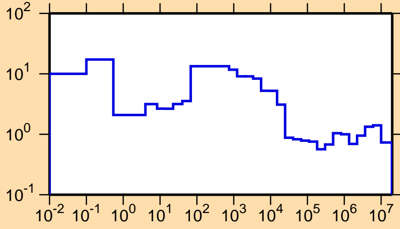
\Delta\sigma/\sigma vs. E for ^{243}\text{Cm}(n,tot.)
