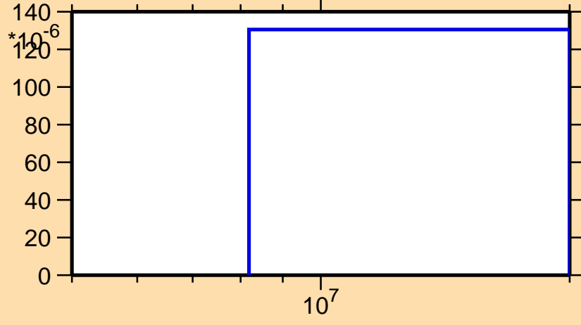
\sigma vs. E for ^{243}\text{Cm}(n,d)
