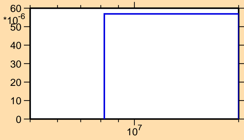
\sigma vs. E for ^{243}\text{Cm}(n,np)
