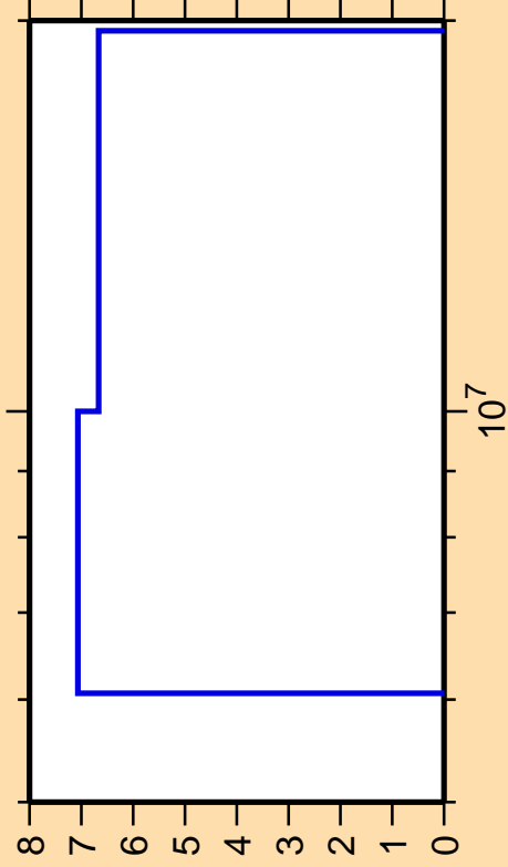
\Delta\sigma/\sigma vs. E for ^{244}\text{Cm}(n,\alpha)
