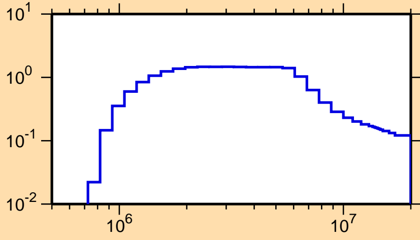
\sigma vs. E for ^{245}\text{Cm}(n,n\text{cont.})
