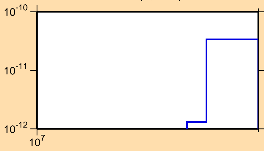
\sigma vs. E for ^{245}\text{Cm}(n,\text{He3})
