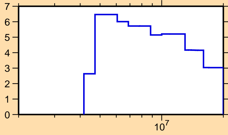
\Delta\sigma/\sigma vs. E for ^{245}\text{Cm}(n,p)
