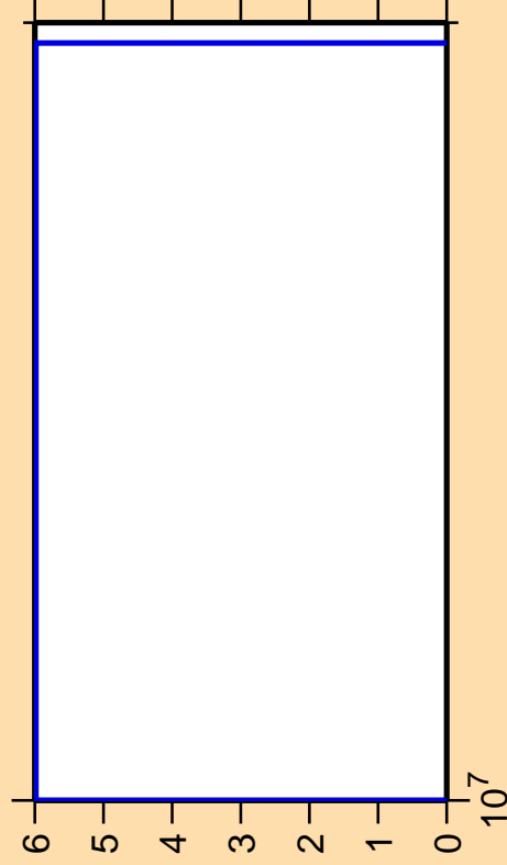
\Delta\sigma/\sigma vs. E for ^{245}\text{Cm}(n,nd)
