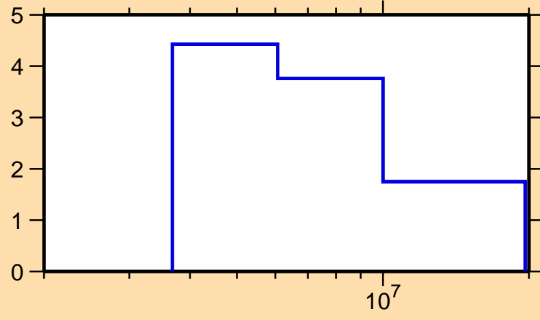
\Delta\sigma/\sigma vs. E for ^{245}\text{Cm}(n,el.)
