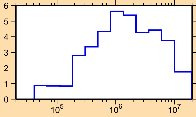
\Delta\sigma/\sigma vs. E for ^{245}\text{Cm}(n,\text{el.})
