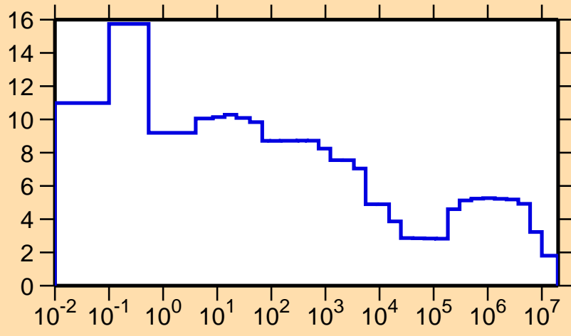
\Delta\sigma/\sigma vs. E for ^{245}\text{Cm}(n,\text{nonel.})
