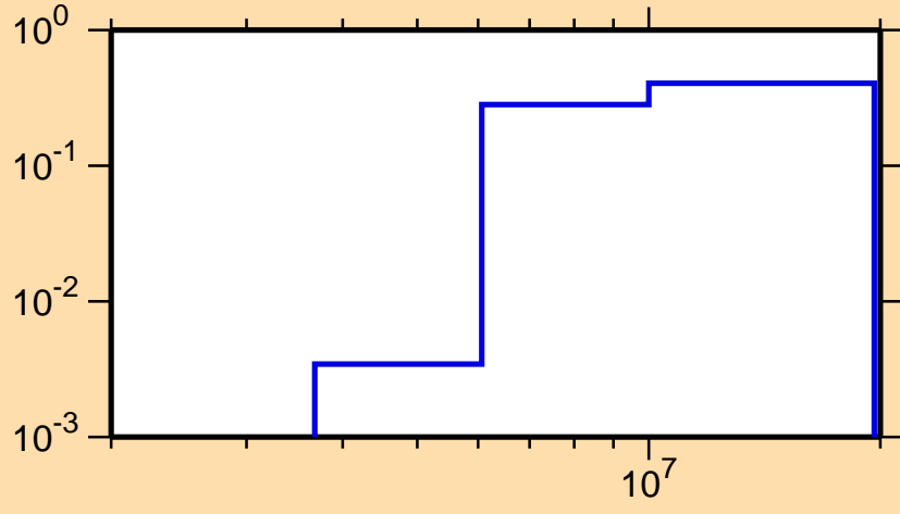
\sigma vs. E for ^{245}\text{Cm}(n,2n)
