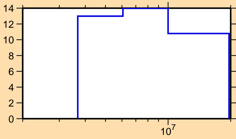
\Delta\sigma/\sigma vs. E for ^{245}\text{Cm}(n,ncont.)
