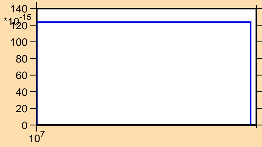
\sigma vs. E for ^{245}\text{Cm}(n,3n\alpha)
