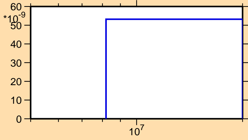
\sigma vs. E for ^{245}\text{Cm}(n,2n\alpha)
