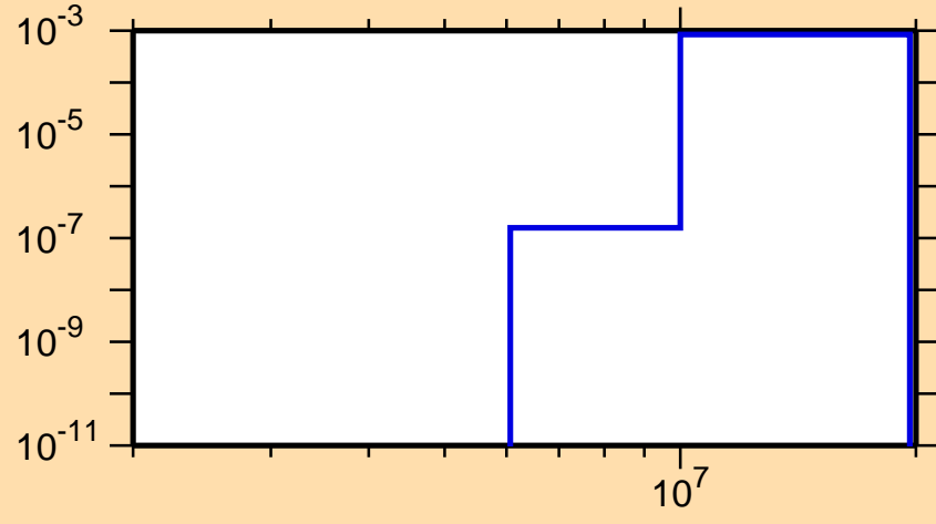
\sigma vs. E for ^{246}\text{Cm}(n,p)
