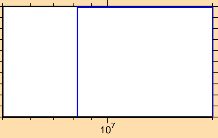
\sigma vs. E for ^{246}\text{Cm}(n,np)
