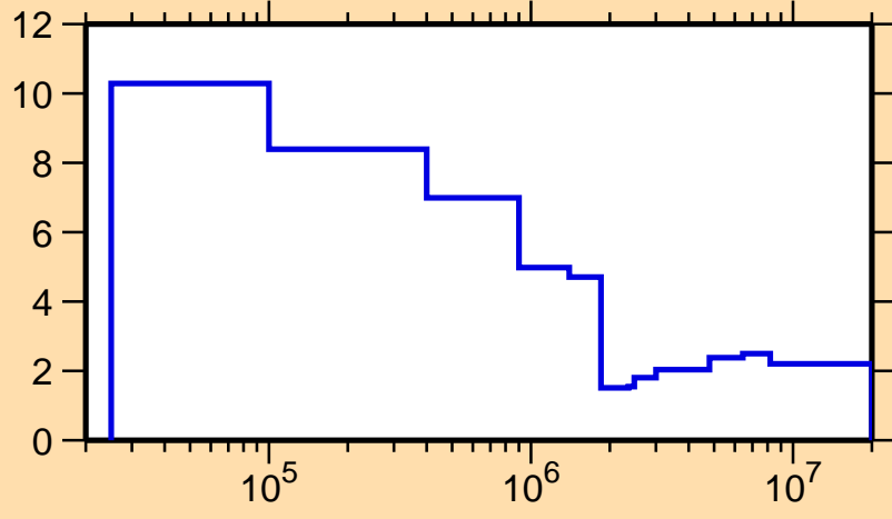
\Delta\sigma/\sigma vs. E for ^{247}\text{Cm}(n,n_1)
