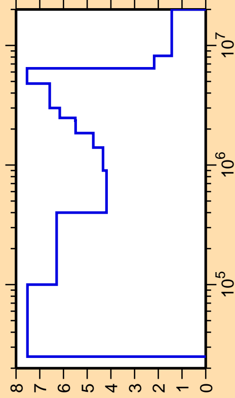
\Delta\sigma/\sigma vs. E for ^{247}\text{Cm}(n,f)
