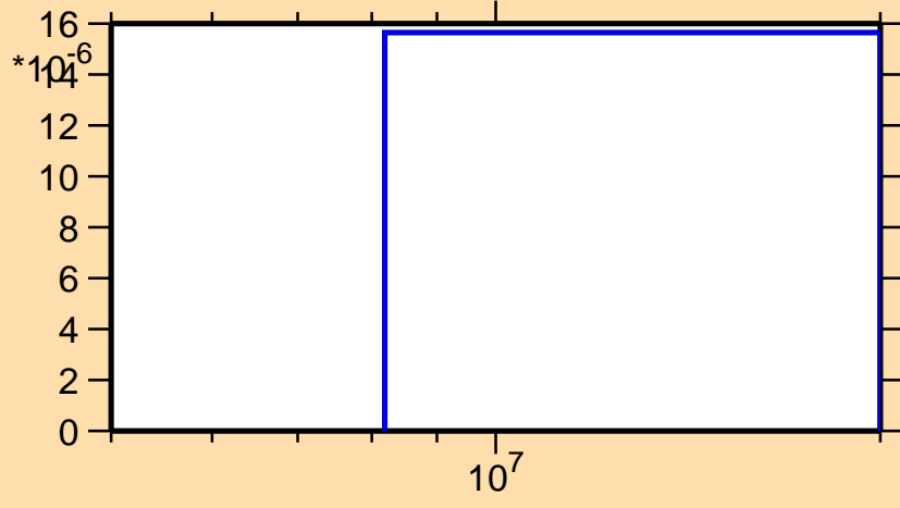
\sigma vs. E for ^{247}\text{Cm}(n,t)
