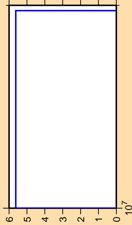
\Delta\sigma/\sigma vs. E for ^{248}\text{Cm}(n,2np)
