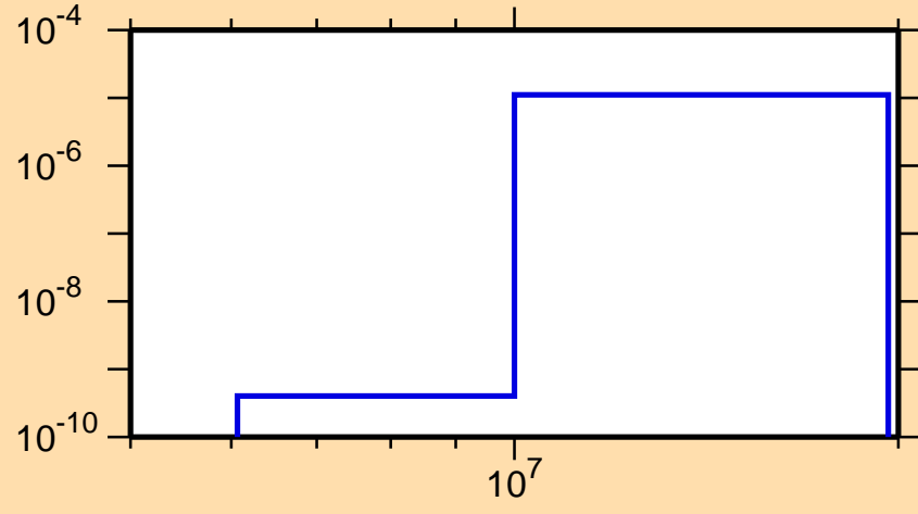
\sigma vs. E for ^{248}\text{Cm}(n,n\alpha)
