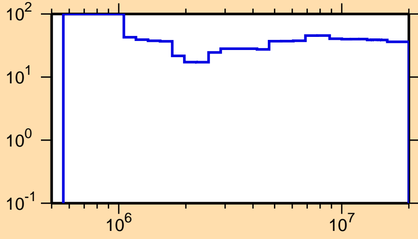
\Delta\sigma/\sigma vs. E for ^{249}\text{Cm}(n,ncont.)
