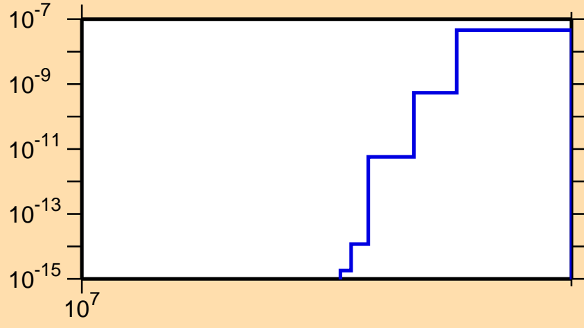
\sigma vs. E for ^{249}\text{Cm}(n,2np)
