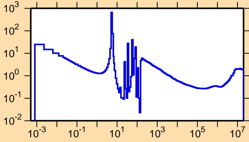
\sigma vs. E for ^{249}\text{Cm}(n,f)
