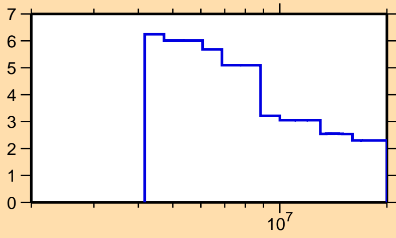
\Delta\sigma/\sigma vs. E for ^{249}\text{Cm}(n,\text{tot.})
