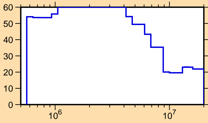
\Delta\sigma/\sigma vs. E for ^{249}\text{Cm}(n,f)
