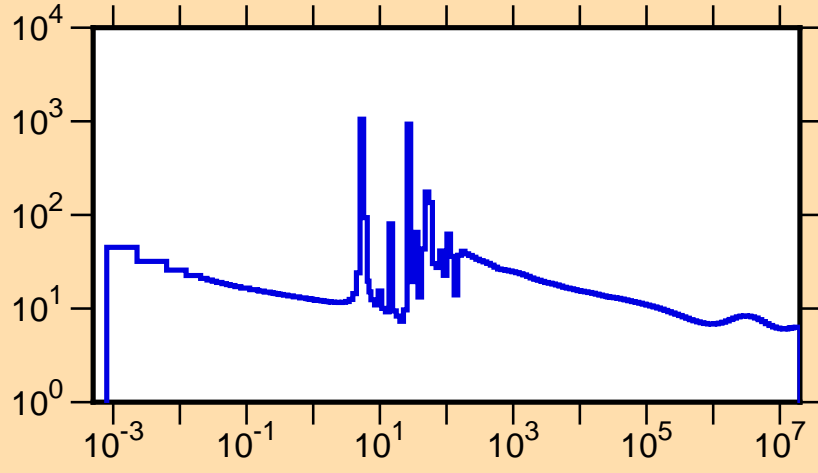
\sigma vs. E for ^{249}\text{Cm}(n,\text{tot.})
