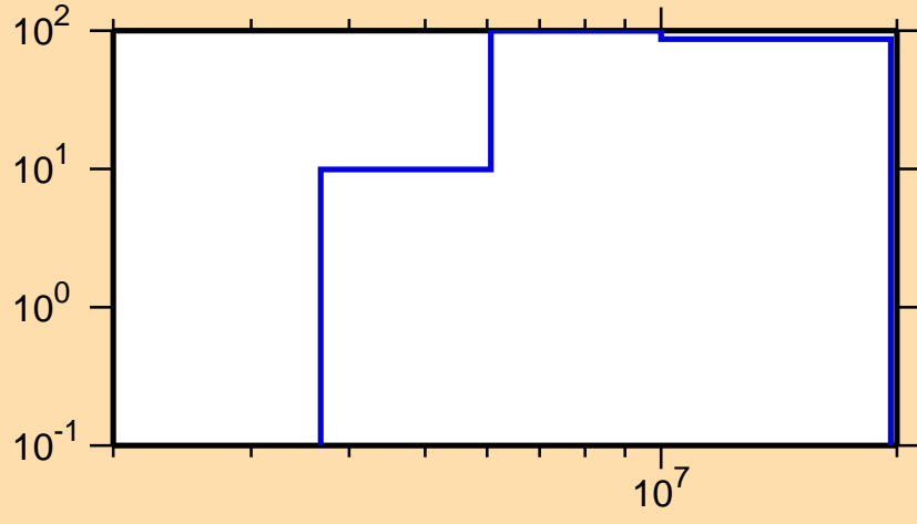
\Delta\sigma/\sigma vs. E for ^{249}\text{Cm}(n,p)
