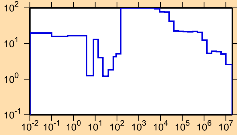
\Delta\sigma/\sigma vs. E for ^{249}\text{Cm}(n,tot.)
