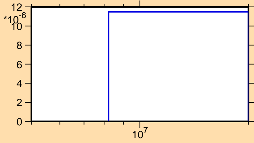
\sigma vs. E for ^{249}\text{Cm}(n,t)
