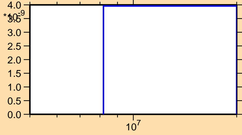
\sigma vs. E for ^{249}\text{Cm}(n,nd)
