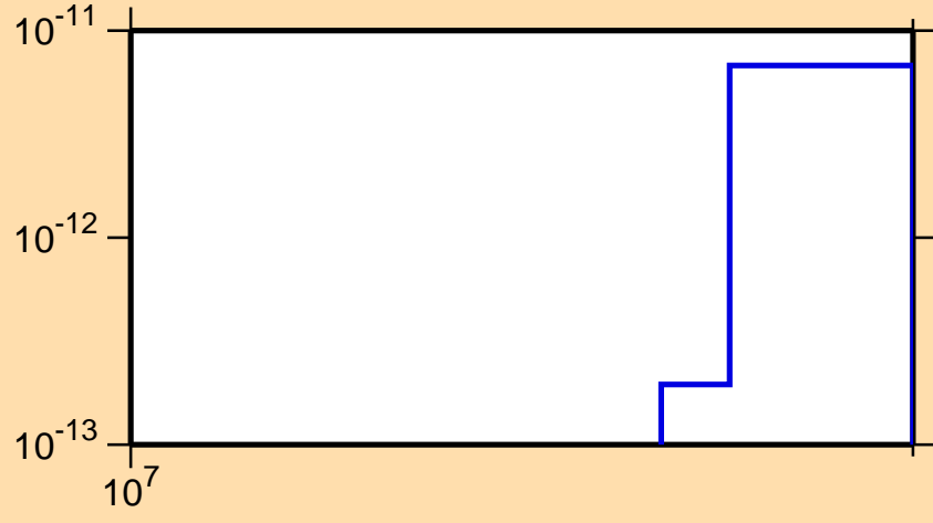
\sigma vs. E for ^{250}\text{Cm}(n,3n\alpha)
