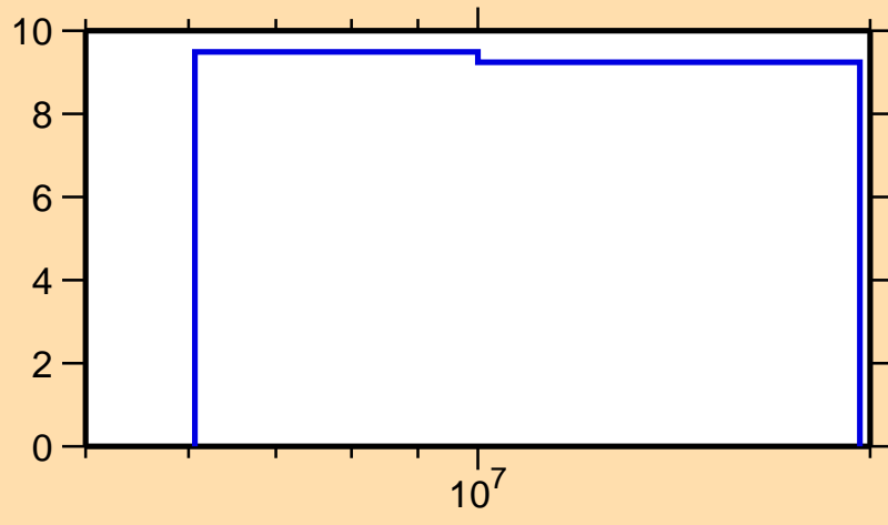
\Delta\sigma/\sigma vs. E for ^{250}\text{Cm}(n,\text{nonel.})
