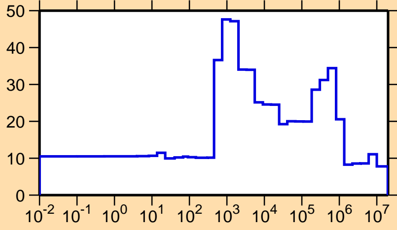
\Delta\sigma/\sigma vs. E for ^{250}\text{Cm}(n,el.)
