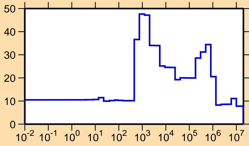
\Delta\sigma/\sigma vs. E for ^{250}\text{Cm}(n,\text{el.})
