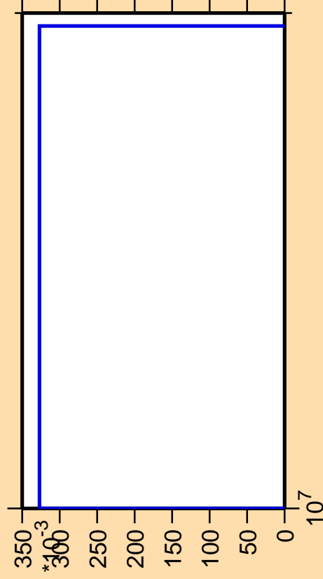
\Delta\sigma/\sigma vs. E for ^{250}\text{Cm}(n,3n\alpha)
