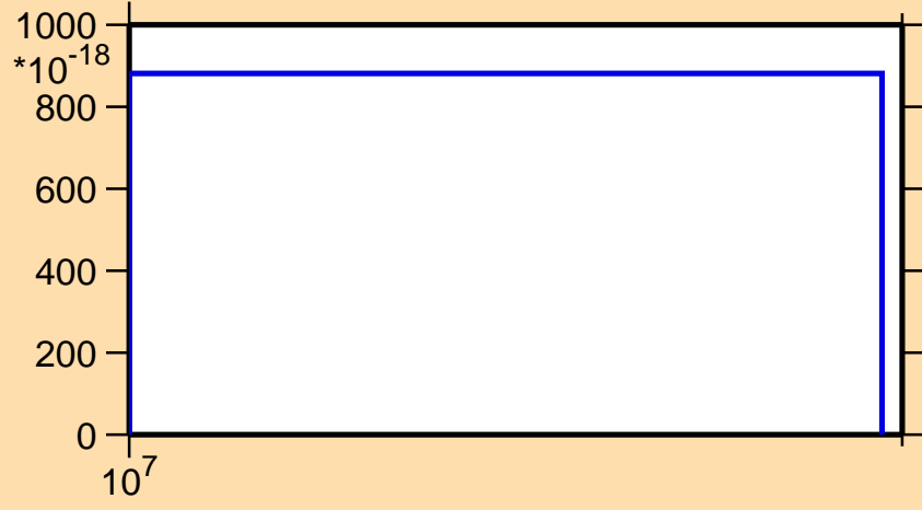
\sigma vs. E for ^{250}\text{Cm}(n,\text{He3})
