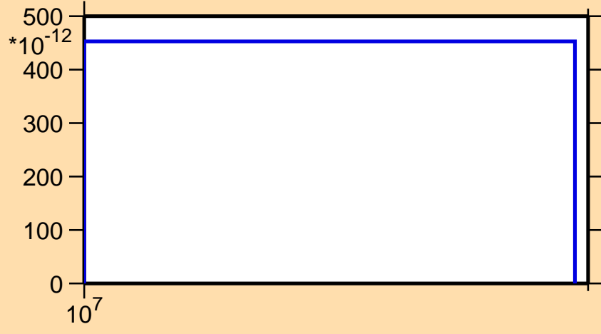
\sigma vs. E for ^{250}\text{Cm}(n,nd)
