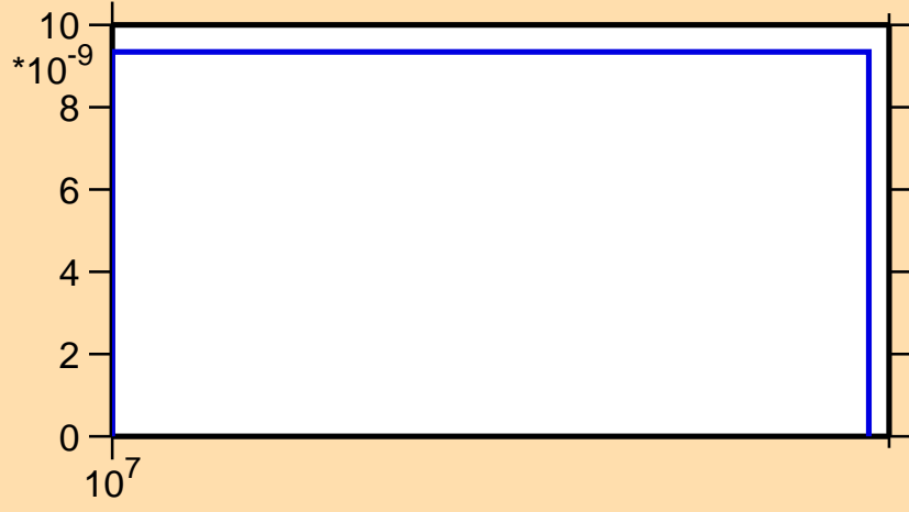
\sigma vs. E for ^{250}\text{Cm}(n,nt)
