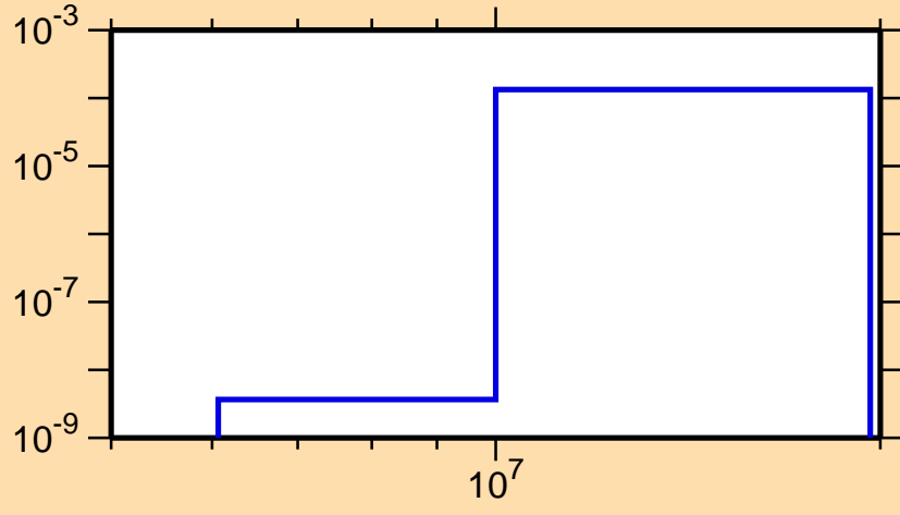
\sigma vs. E for ^{250}\text{Cm}(n,p)
