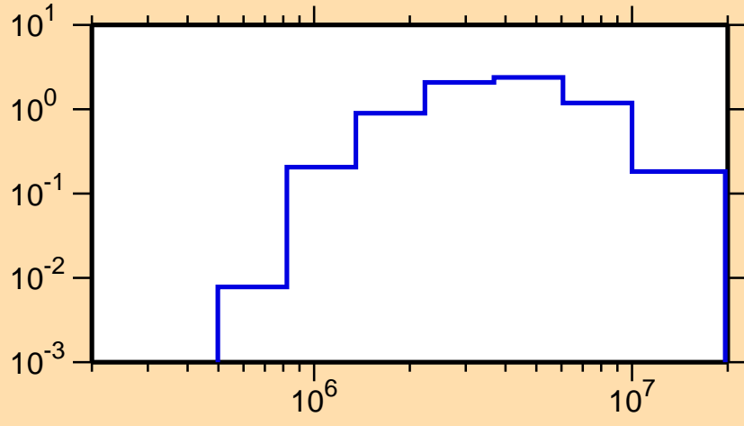
\sigma vs. E for ^{250}\text{Cm}(n,n\text{cont.})
