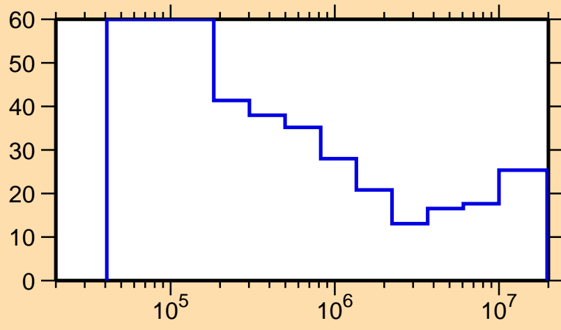
\Delta\sigma/\sigma vs. E for ^{250}\text{Cm}(n,\text{inel.})
