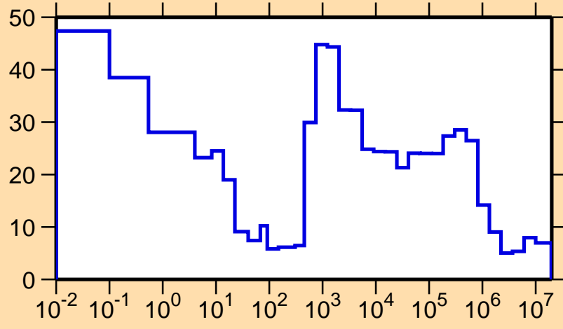
\Delta\sigma/\sigma vs. E for ^{250}\text{Cm}(n,\text{tot.})
