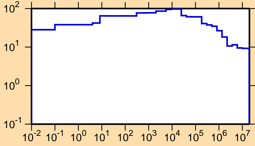
\Delta\sigma/\sigma vs. E for ^{250}\text{Cm}(n,\text{nonel.})
