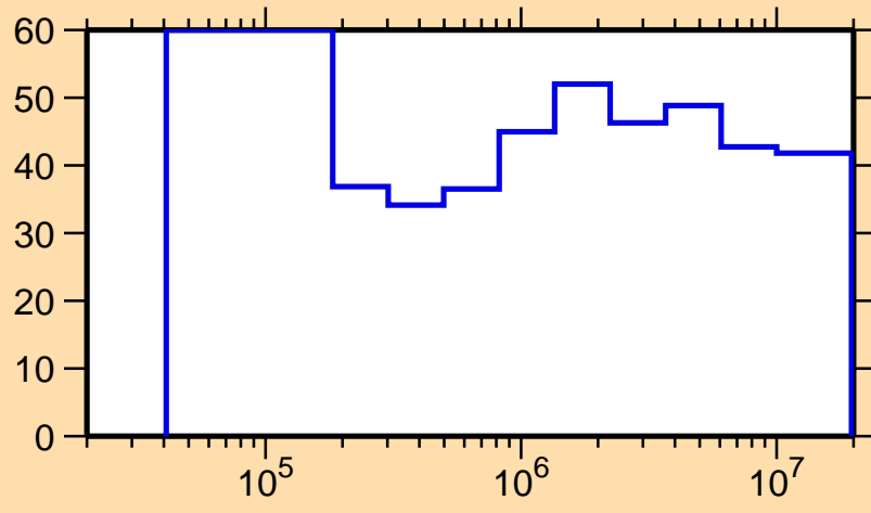
\Delta\sigma/\sigma vs. E for ^{250}\text{Cm}(n,n_1)
