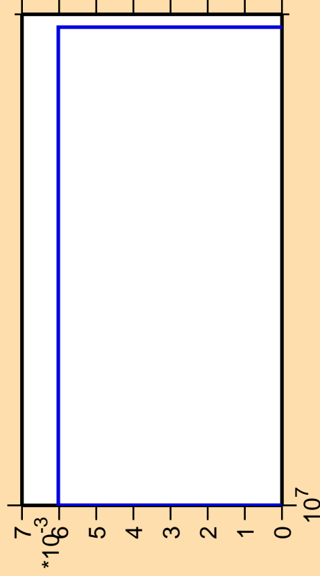
\Delta\sigma/\sigma vs. E for ^{250}\text{Cm}(n,\text{He3})
