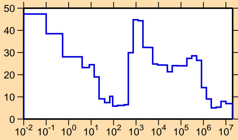
\Delta\sigma/\sigma vs. E for ^{250}\text{Cm}(n,tot.)
