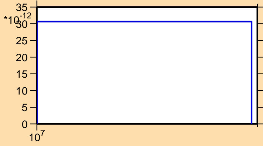
\sigma vs. E for ^{250}\text{Cm}(n,2np)
