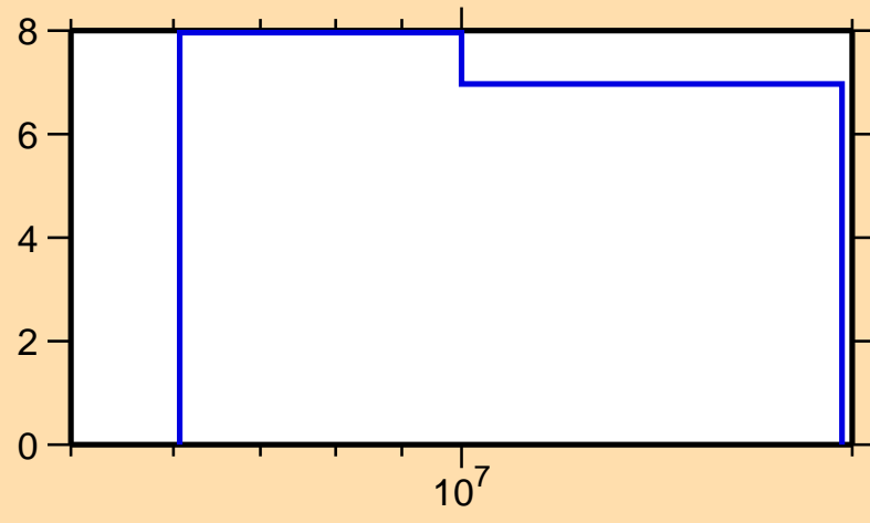
\Delta\sigma/\sigma vs. E for ^{250}\text{Cm}(n,\text{tot.})
