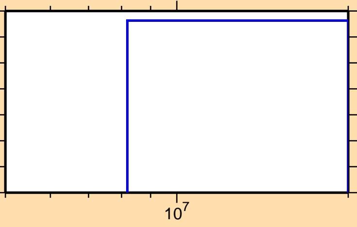
\sigma vs. E for ^{250}\text{Cm}(n,d)
