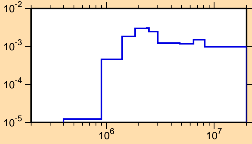
\sigma vs. E for ^{250}\text{Cm}(n,n_4)
