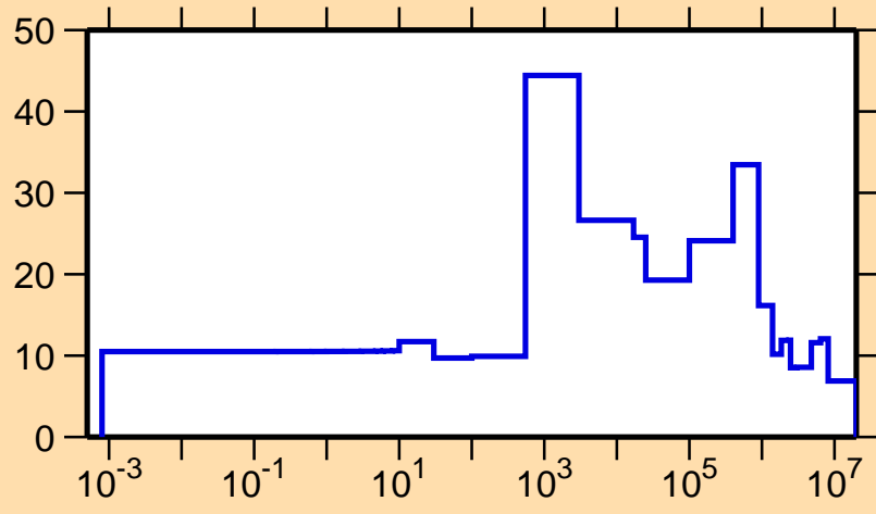
\Delta\sigma/\sigma vs. E for ^{250}\text{Cm}(n,el.)
