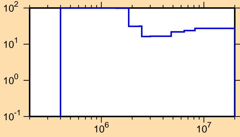
\Delta\sigma/\sigma vs. E for ^{250}\text{Cm}(n,n\text{cont.})
