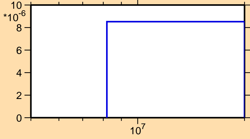
\sigma vs. E for ^{250}\text{Cm}(n,t)
