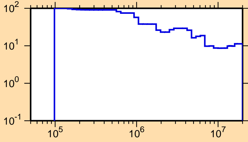
\Delta\sigma/\sigma vs. E for ^{251}\text{Cm}(n,n\text{cont.})
