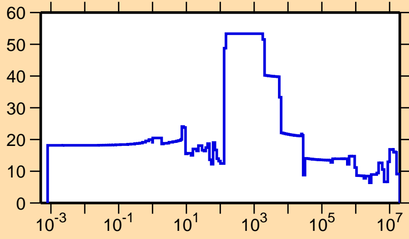
\Delta\sigma/\sigma vs. E for ^{251}\text{Cm}(n,el.)
