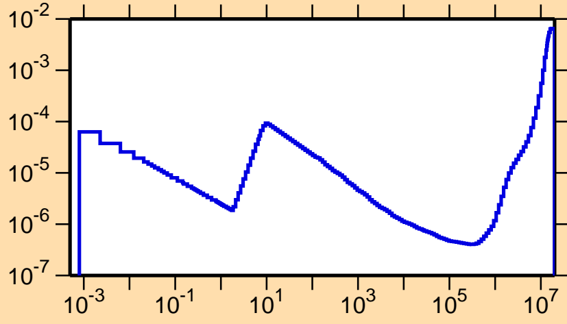
\sigma vs. E for ^{251}\text{Cm}(n,\alpha)
