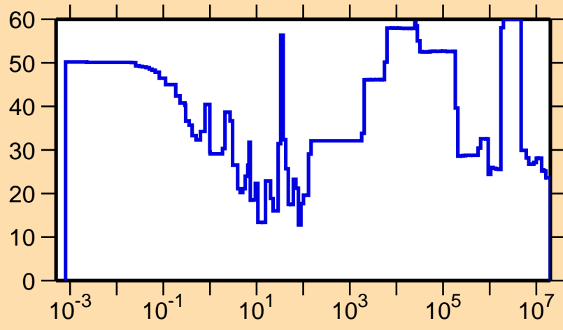
\Delta\sigma/\sigma vs. E for ^{251}\text{Cm}(n,\gamma)
