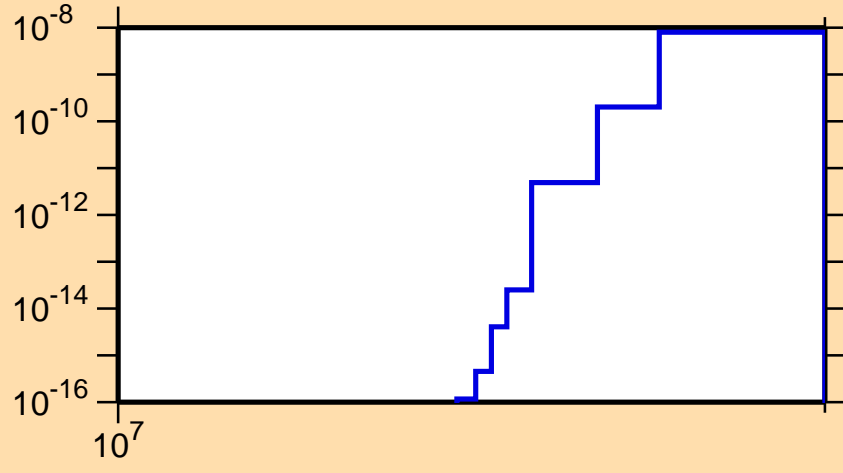
\sigma vs. E for ^{251}\text{Cm}(n,2np)
