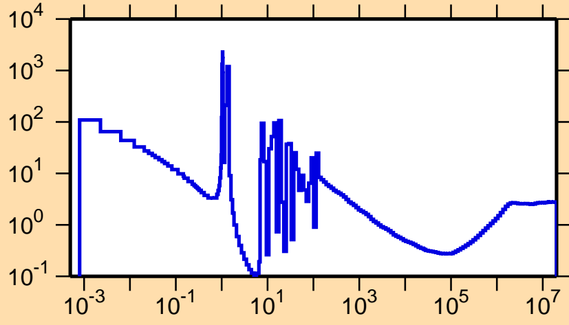
\sigma vs. E for ^{251}\text{Cm}(n,\text{nonel.})
