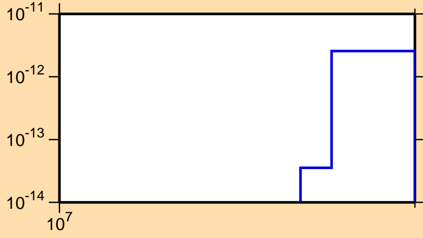
\sigma vs. E for ^{251}\text{Cm}(n,\text{He}3)
