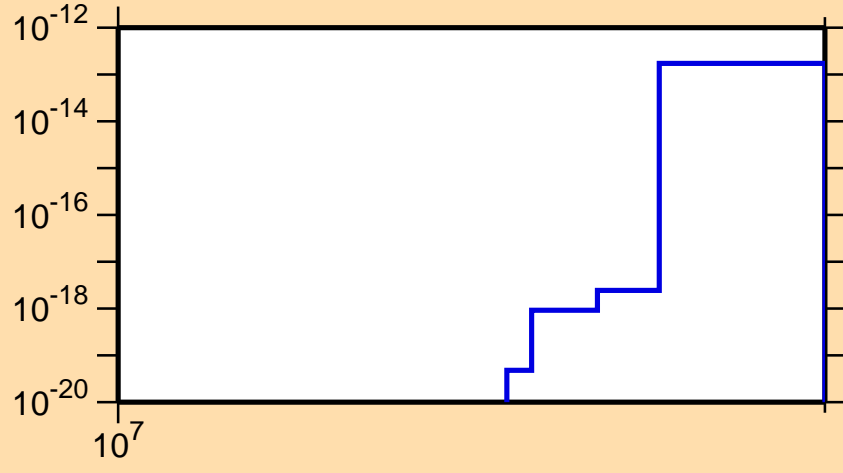
\sigma vs. E for ^{251}\text{Cm} (mt 11)
