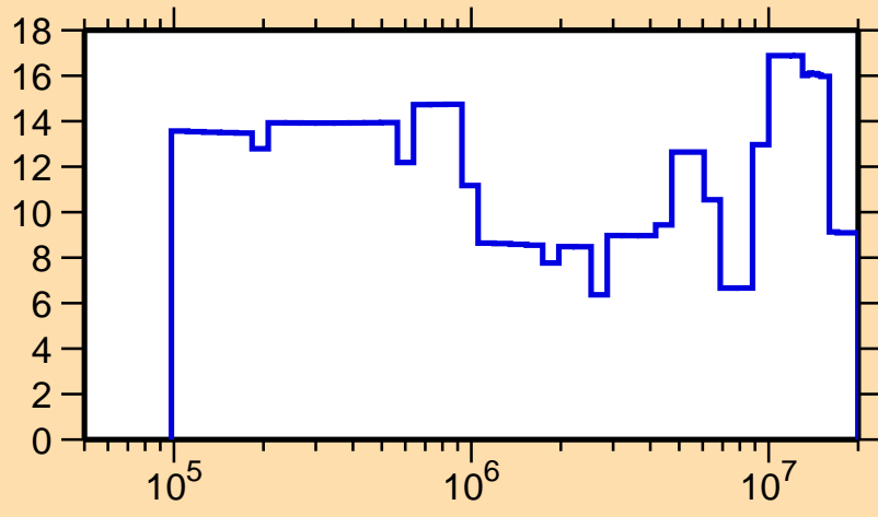
\Delta\sigma/\sigma vs. E for ^{251}\text{Cm}(n,\text{el.})
