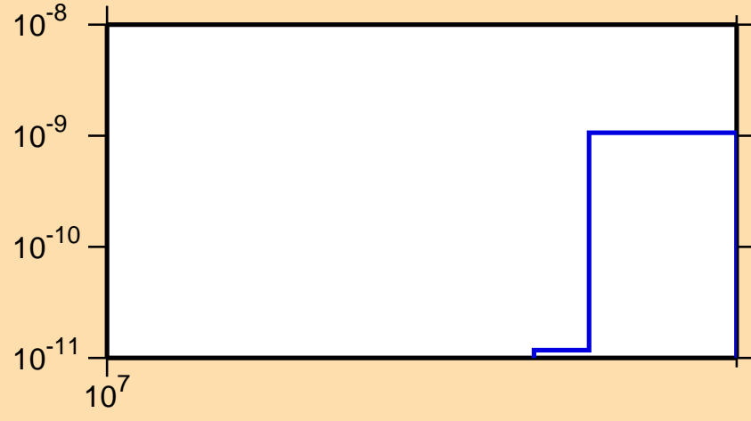
\sigma vs. E for ^{251}\text{Cm}(n,3n\alpha)
