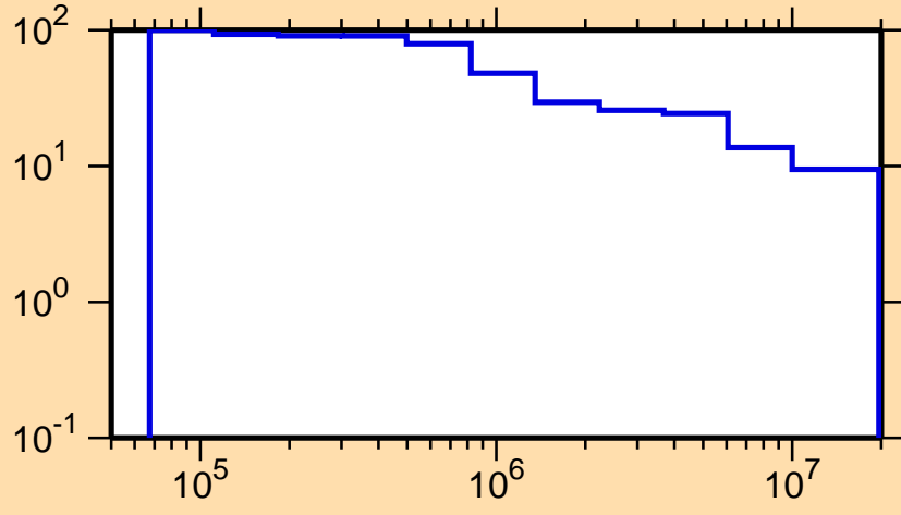
\Delta\sigma/\sigma vs. E for ^{251}\text{Cm}(n,ncont.)
