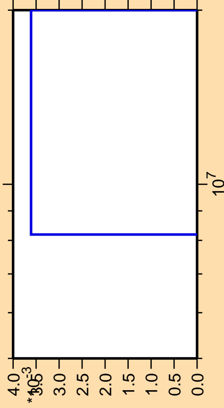
\Delta\sigma/\sigma vs. E for ^{251}\text{Cm}(\text{mt } 11)
