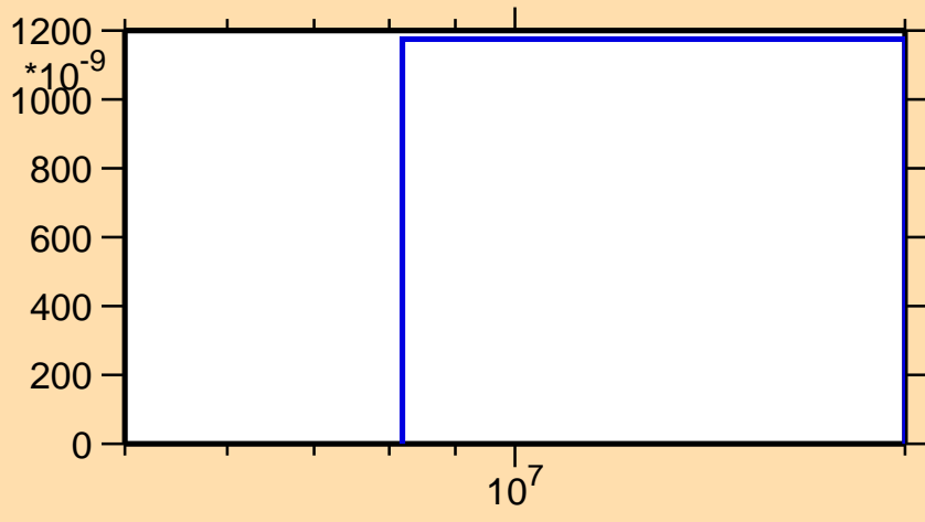
\sigma vs. E for ^{251}\text{Cm}(n,np)
