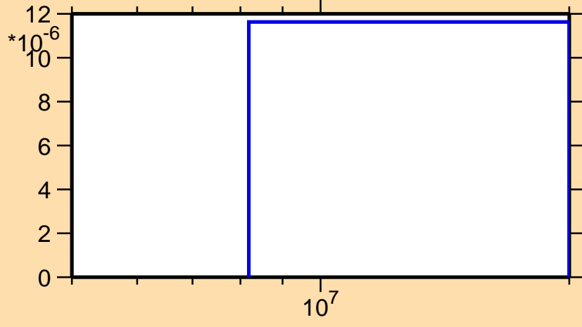
\sigma vs. E for ^{251}\text{Cm}(n,t)
