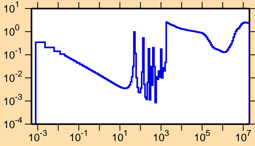
\sigma vs. E for ^{252}\text{Cm}(n,f)
