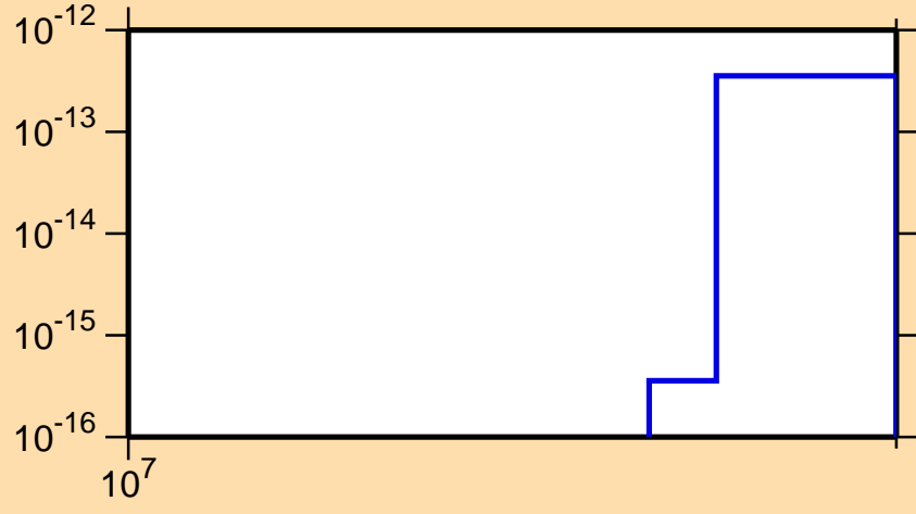
\sigma vs. E for ^{252}\text{Cm}(n,2np)
