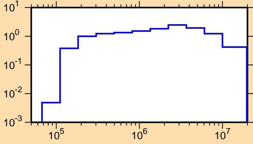
\sigma vs. E for ^{252}\text{Cm}(n,\text{inel.})
