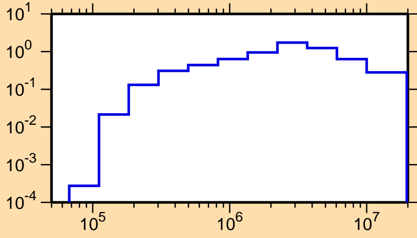
\sigma vs. E for ^{252}\text{Cm}(n,n_1)
