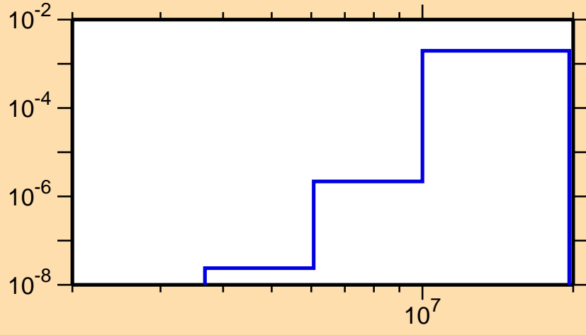
\sigma vs. E for ^{252}\text{Cm}(n,n\alpha)
