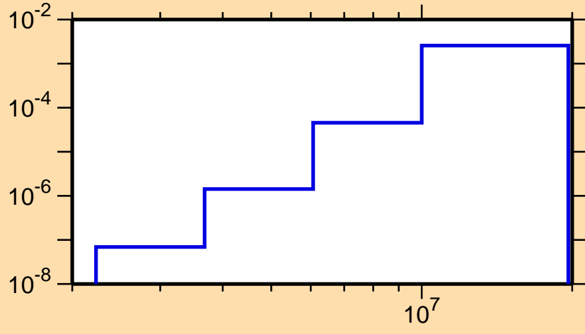
\sigma vs. E for ^{252}\text{Cm}(n,\alpha)
