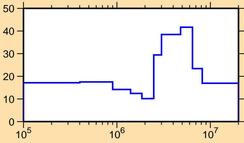
\Delta\sigma/\sigma vs. E for ^{252}\text{Cm}(n,\text{inel.})
