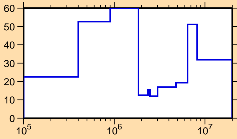
\Delta\sigma/\sigma vs. E for ^{252}\text{Cm}(n,\text{el.})
