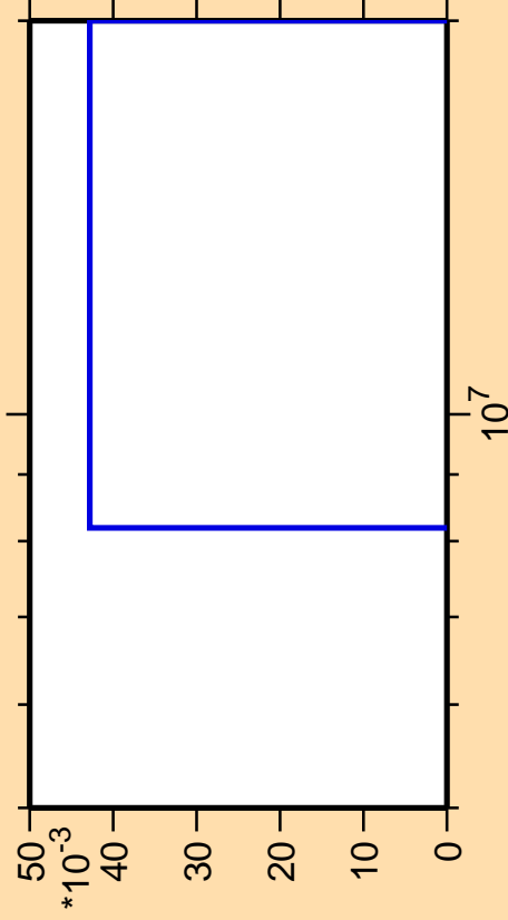
\Delta\sigma/\sigma vs. E for ^{252}\text{Cm}(n,3n\alpha)
