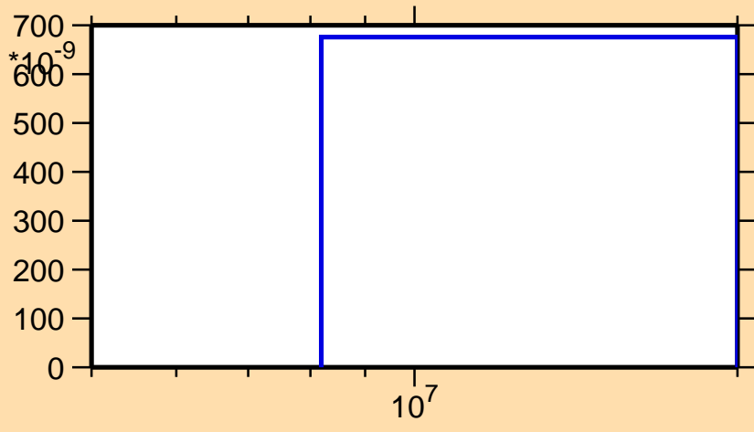
\sigma vs. E for ^{252}\text{Cm}(n,d)
