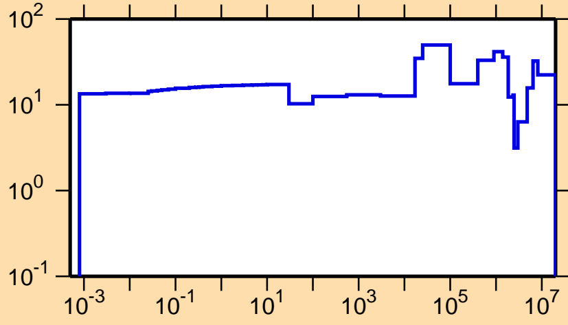
\Delta\sigma/\sigma vs. E for ^{252}\text{Cm}(n,tot.)
