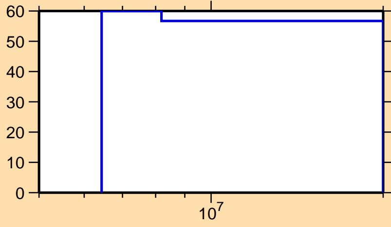
\Delta\sigma/\sigma vs. E for ^{252}\text{Cm}(n,ncont.)
