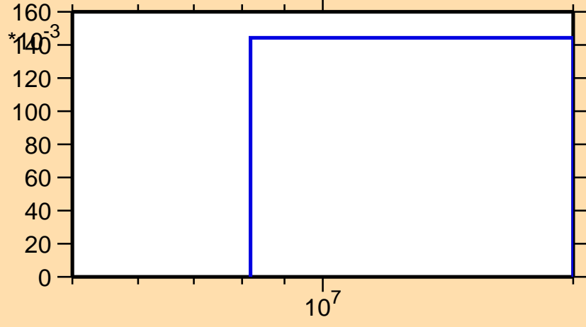
\sigma vs. E for ^{252}\text{Cm}(n,3n)
