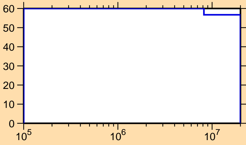
\Delta\sigma/\sigma vs. E for ^{252}\text{Cm}(n,n\text{cont.})
