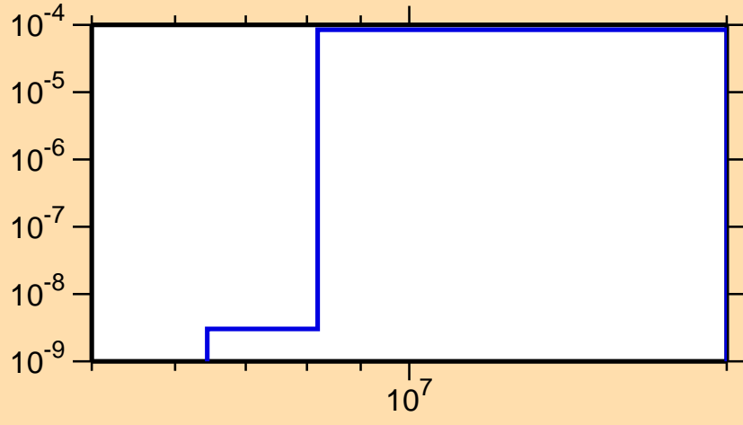
\sigma vs. E for ^{252}\text{Cm}(n,p)
