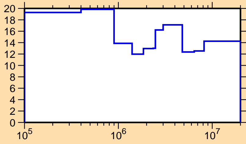
\Delta\sigma/\sigma vs. E for ^{252}\text{Cm}(n,\text{nonel.})
