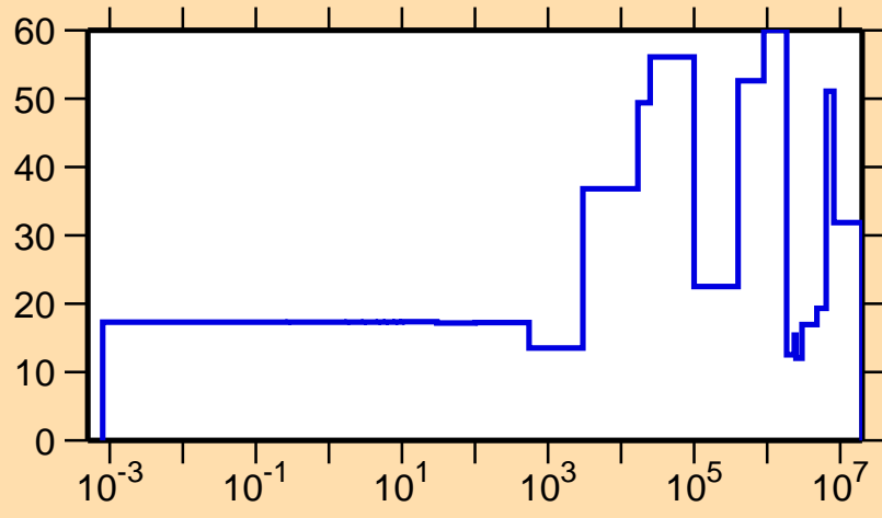
\Delta\sigma/\sigma vs. E for ^{252}\text{Cm}(n,el.)
