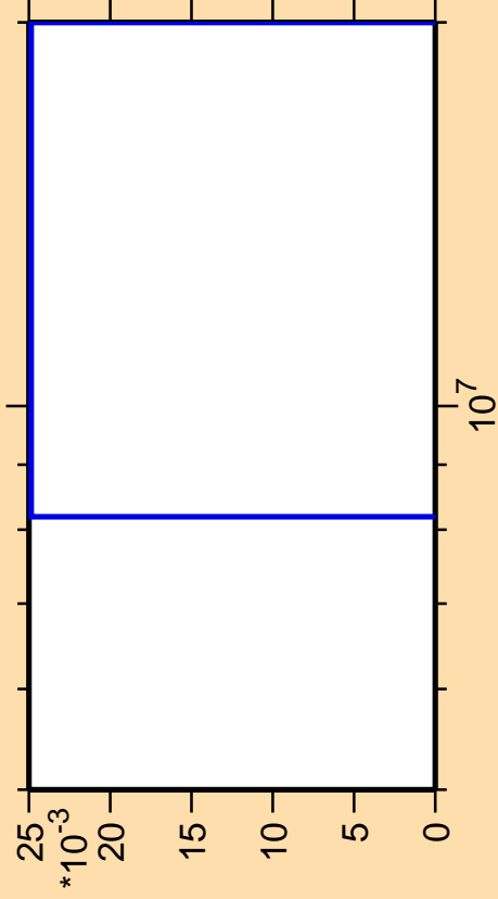
\Delta\sigma/\sigma vs. E for ^{252}\text{Cm}(n,2np)
