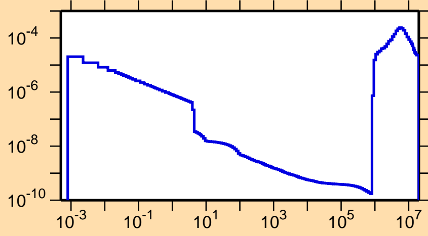
\sigma vs. E for ^{283}\gamma
