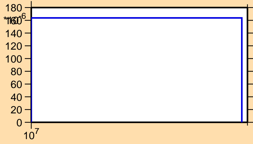
\sigma vs. E for ^{283}\alpha )
