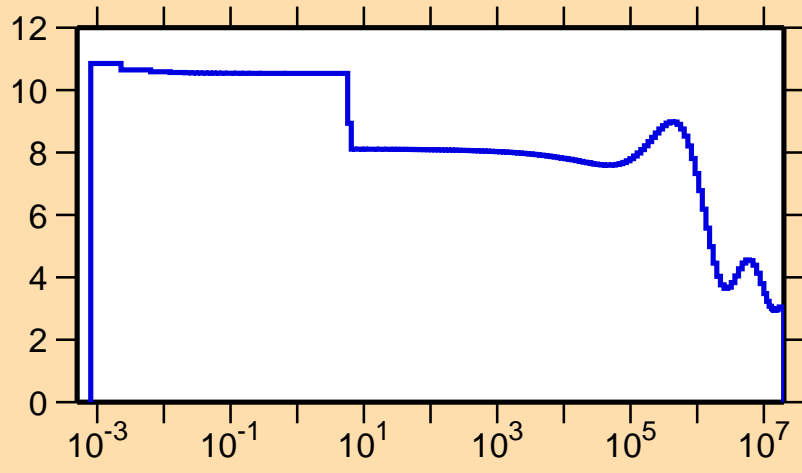
\sigma vs. E for ^{285}
