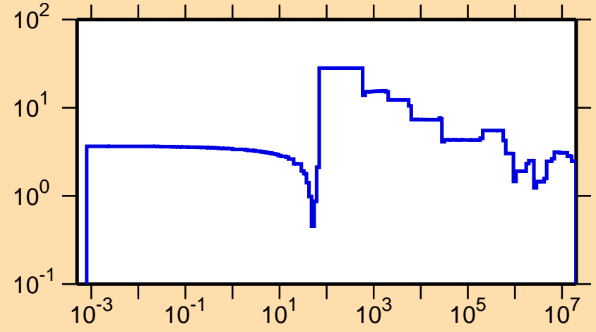
\Delta\sigma/\sigma vs. E for ^{54}\text{Co}(n,\text{tot.})
