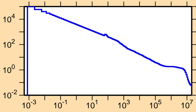
\sigma vs. E for ^{54}\text{Co}(n,p)
