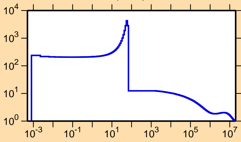
\sigma vs. E for ^{54}\text{Co}(n,\text{el.})
