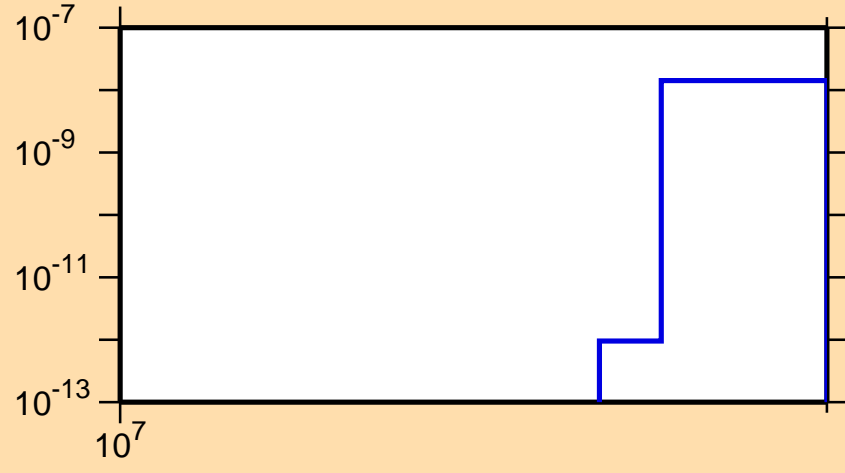
\sigma vs. E for ^{54}\text{Co} (mt 45)
