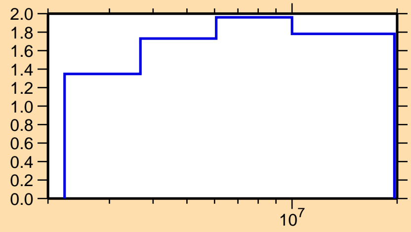
\Delta\sigma/\sigma vs. E for ^{54}\text{Co}(n,n\text{onel.})
