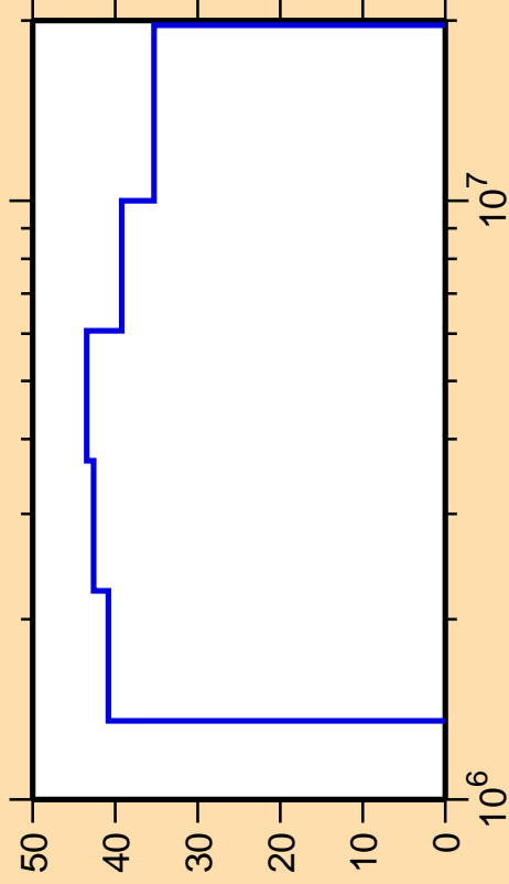
\Delta\sigma/\sigma vs. E for ^{54}\text{Co}(n,n_4)
