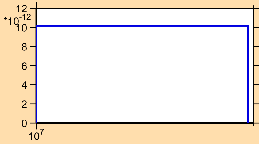
\sigma vs. E for ^{54}\text{Co} (mt 34)
