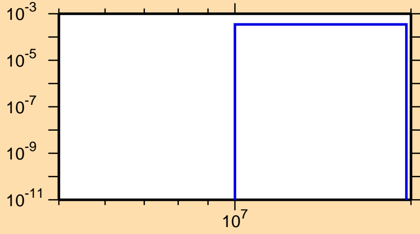
\sigma vs. E for ^{54}\text{Co}(n,pd)
