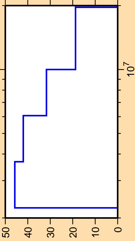
\Delta\sigma/\sigma vs. E for ^{54}\text{Co}(n,n\text{cont.})
