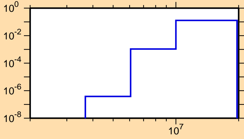
\sigma vs. E for ^{54}\text{Co}(n,p\alpha)
