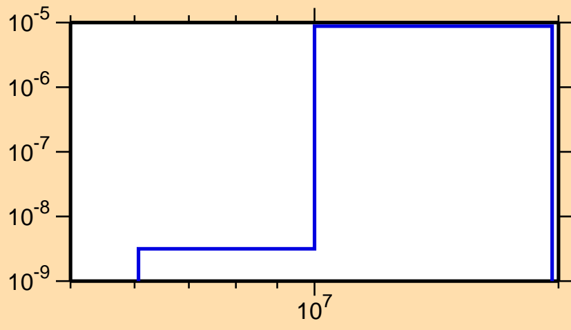
\sigma vs. E for ^{54}\text{Co}(n,t)
