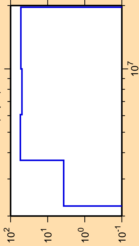
\Delta\sigma/\sigma vs. E for ^{54}\text{Co}(n,p\alpha)
