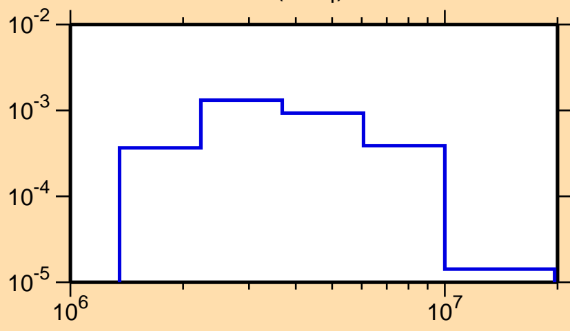
\sigma vs. E for ^{54}\text{Co}(n,n_4)
