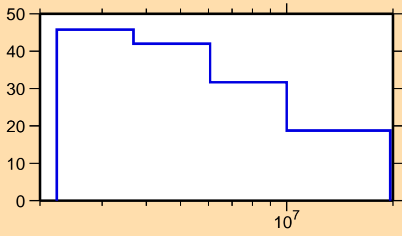
\Delta\sigma/\sigma vs. E for ^{54}\text{Co}(n,n\text{cont.})
