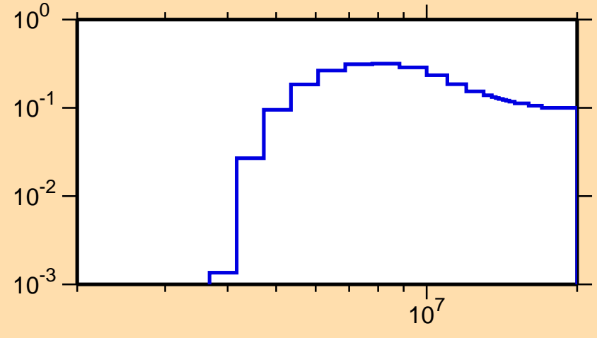
\sigma vs. E for ^{55}\text{Co}(n,n\text{cont.})
