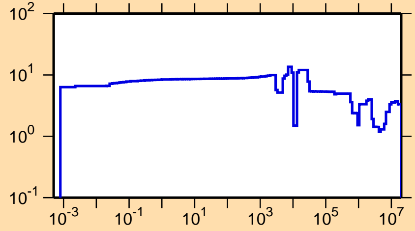
\Delta\sigma/\sigma vs. E for ^{55}\text{Co}(n,\text{tot.})
